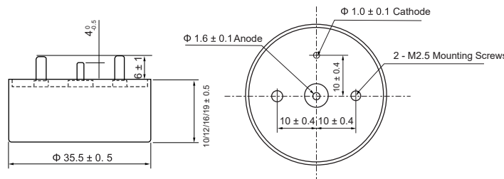
Mounting Dimensional Diagram of the THC2W Φ35.5 x 10/12/16/19 ( Type B )
