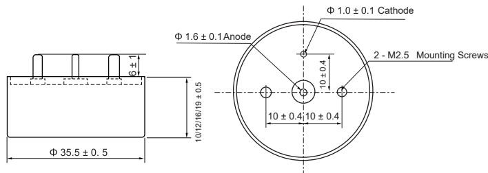
Mounting Dimensional Diagram of the THC2W Φ35.5 x 10/12/16/19 ( Type A )
