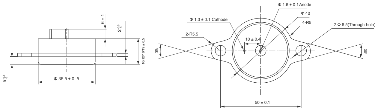
Mounting Dimensional Diagram of the THC2FB Φ35.5 x 10/12/16/19
