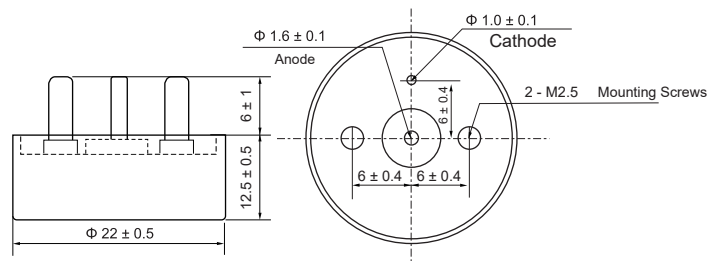
Mounting Dimensional Diagram of the THC1W Φ22 x 12.5
