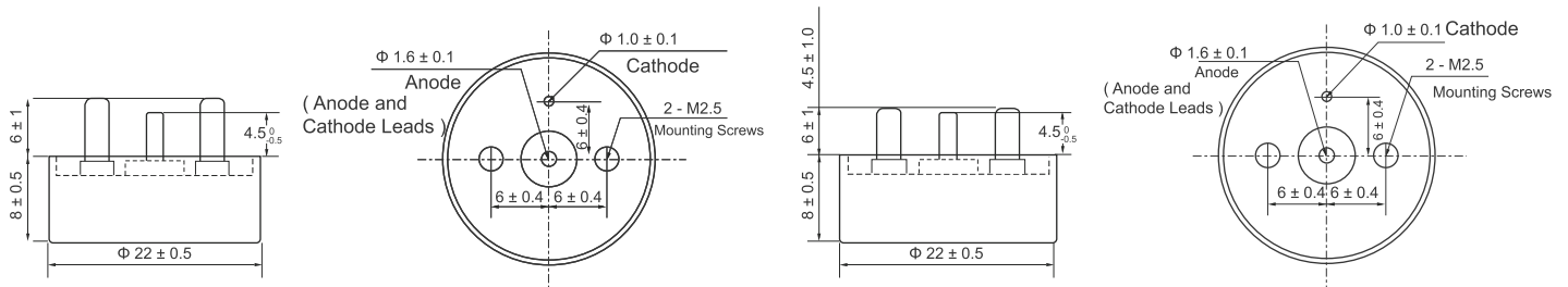
Mounting Dimensional Diagram of the HTHC1W Φ22 x 8 ( Type A )
