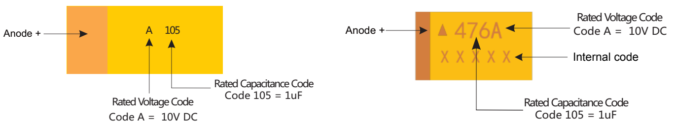
Voltage Code Table for Chip Tantalum Capacitors
