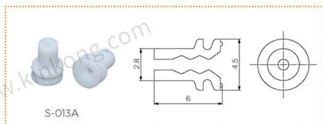
wire seal
