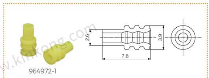
wire seal
