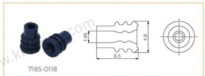
wire seal
