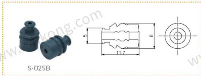
wire seal
