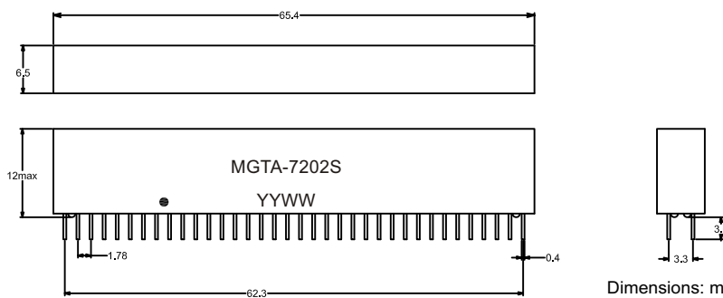
Dimensions: mm Unless otherwise specified, all tolerances are ±0.25
