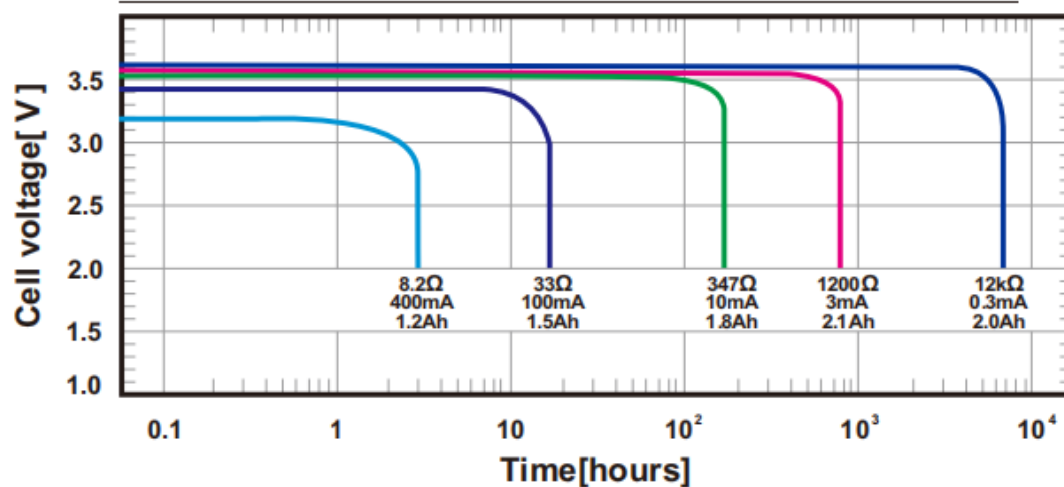
Typical Discharge Profiles at +23\pm 2^{\circ}\text{C}
