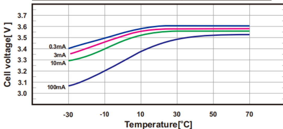
Voltage Plateau Versus Current and Temperature
