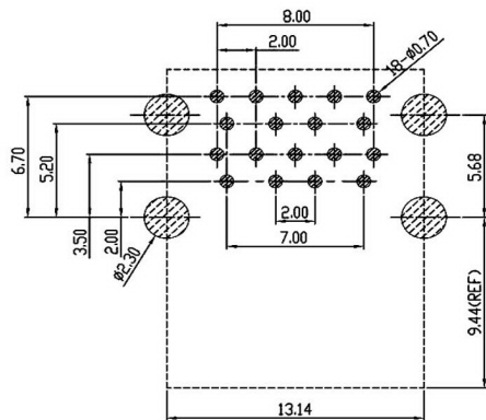
PCB LAYOUT REFERENCE
