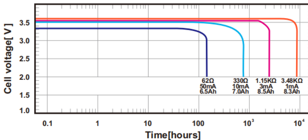
Typical Discharge Profiles at +23±2°C
