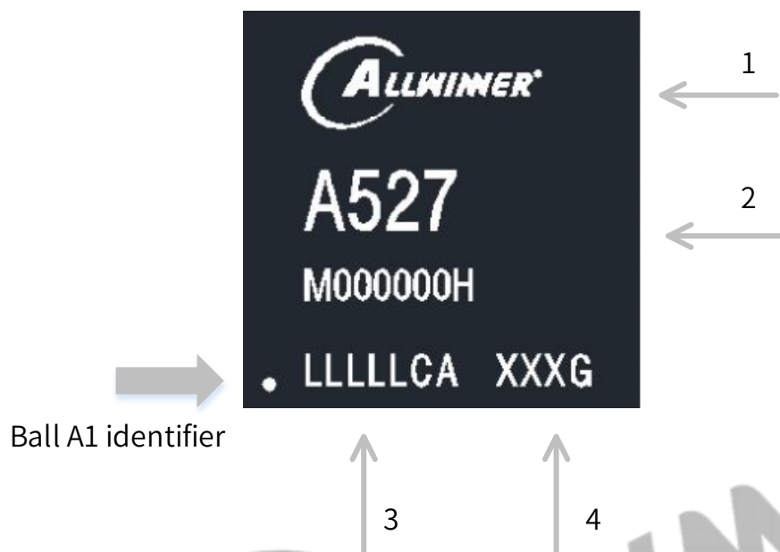
Figure 12-4 A527M000000H Marking
