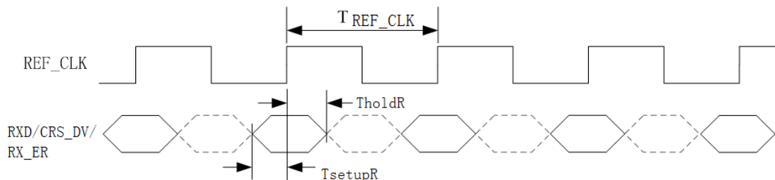
Figure 6-39 RMII Transmit Timing
