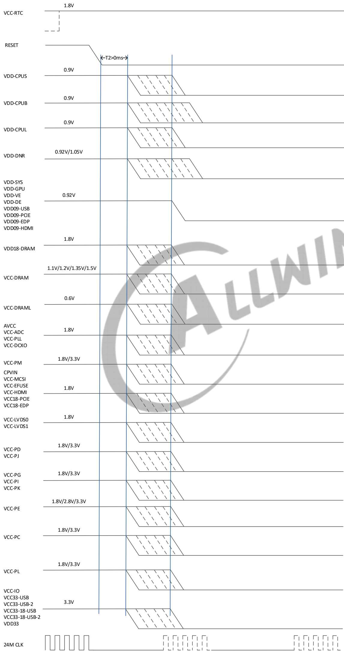
Figure 6-48 Power-off Timing
