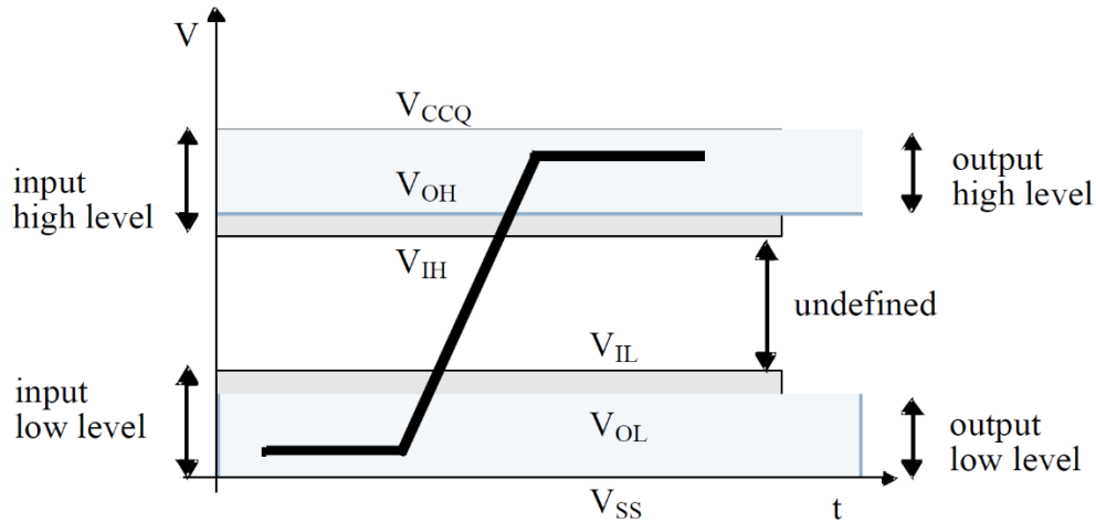
Figure 6-2 SMHC Voltage Waveform
