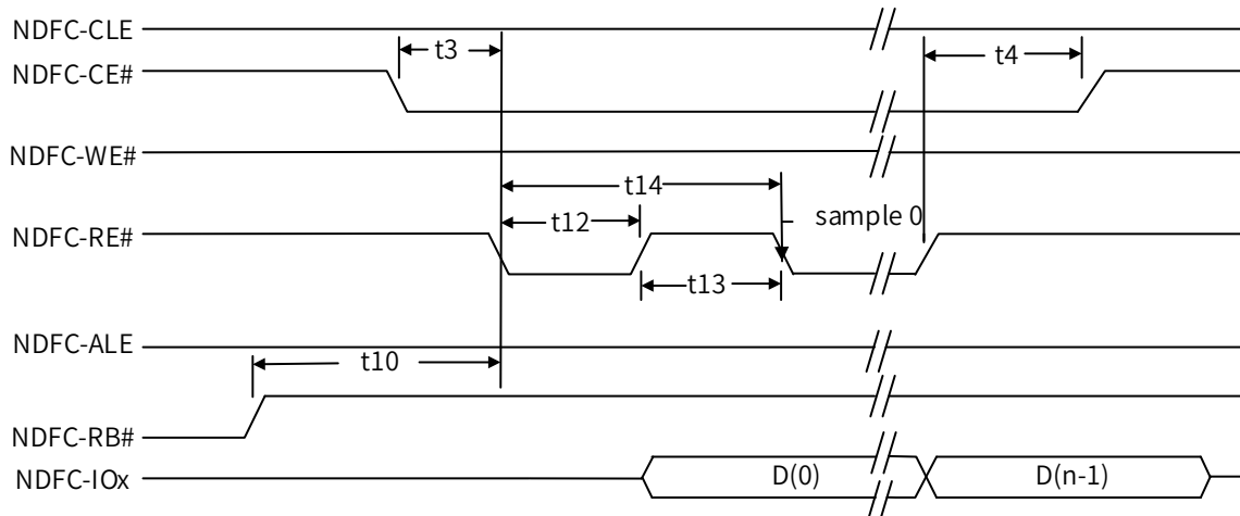
Figure 6-4 EDO Type Serial Access after Read Cycle Timing (SAM1)
