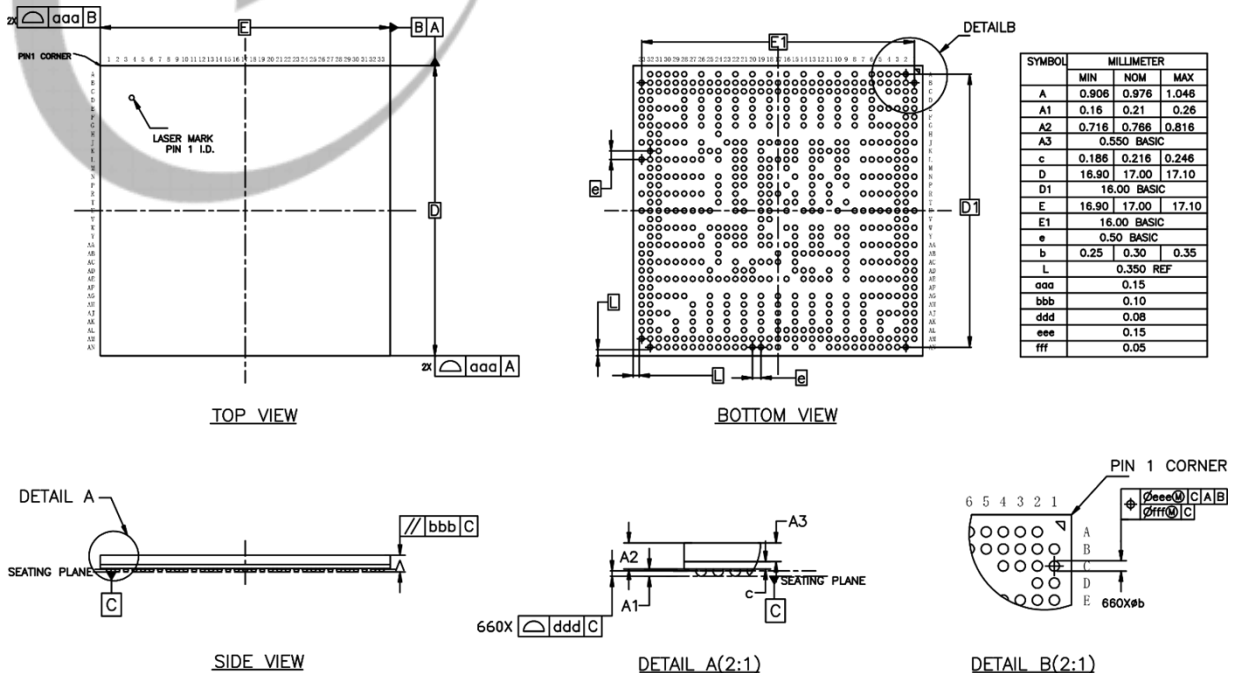
Figure 8-3 Package Dimension
