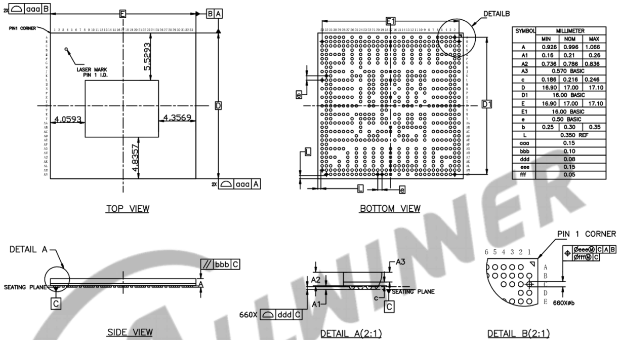
Figure 8-2 Package Dimension
