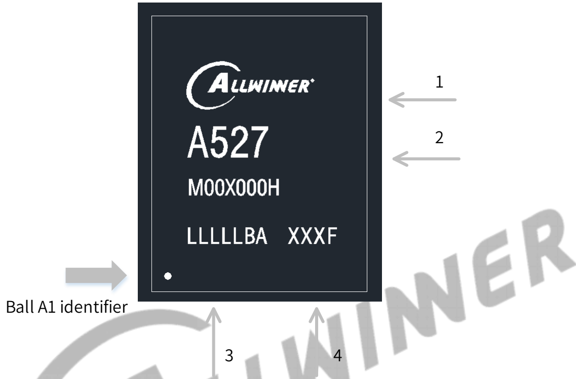
Figure 12-3 A527M00X000H Marking
