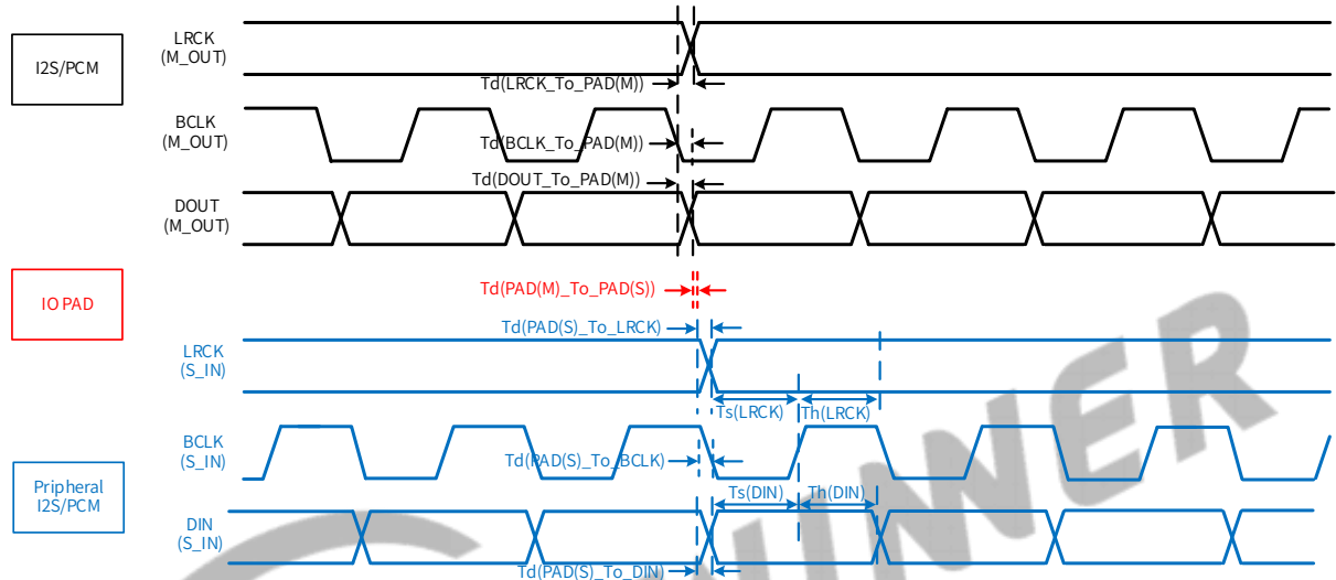
Figure 6-44 Data Output Timing of I2S/PCM in Master Mode
