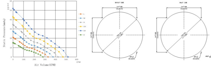
Fan Performance Curve
