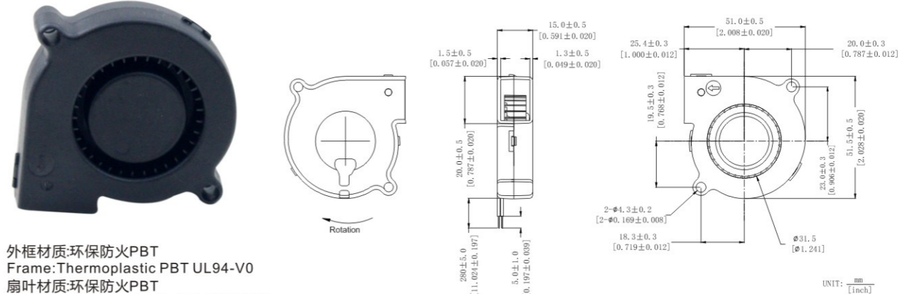
DIMENSIONS DRAWING
