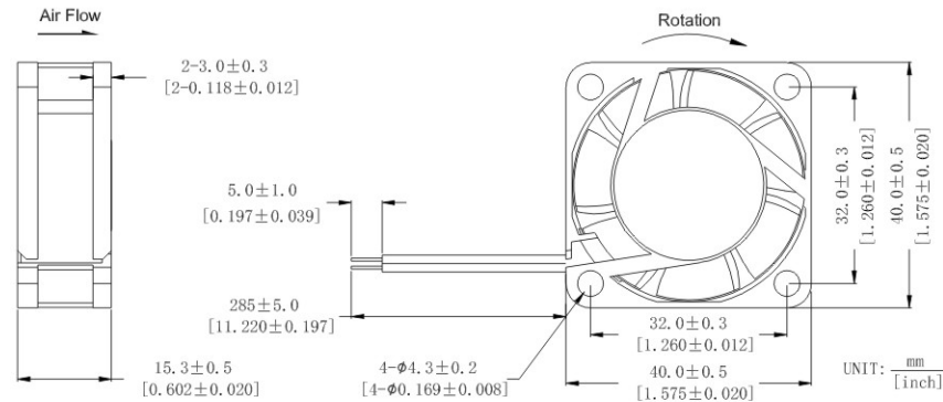
DIMENSIONS DRAWING
