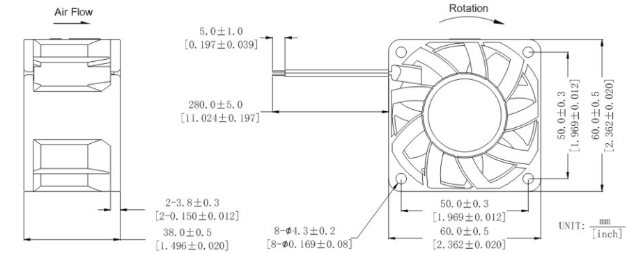
DIMENSIONS DRAWING
