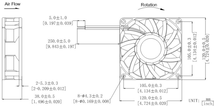
DIMENSIONS DRAWING
