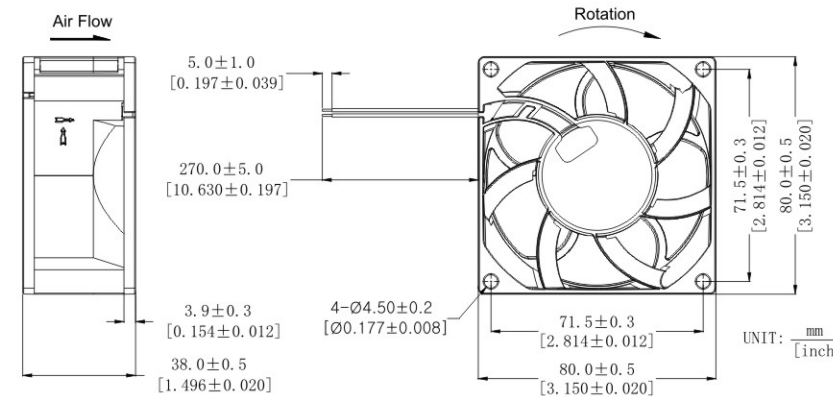
DIMENSIONS DRAWING
