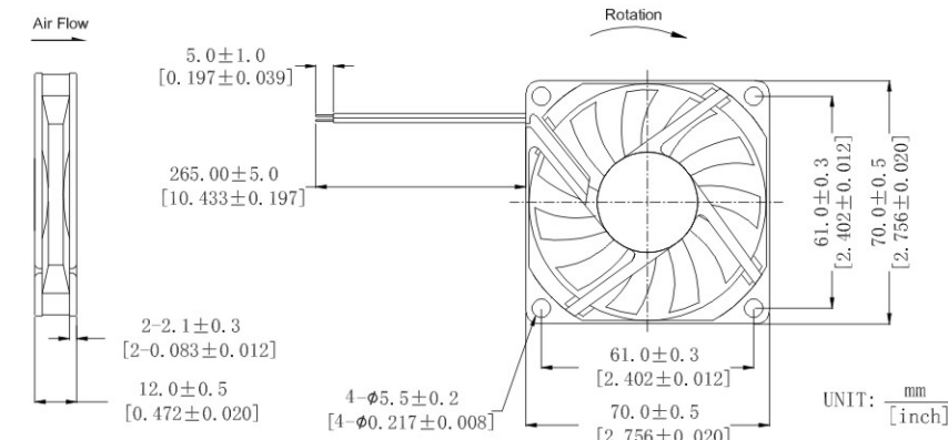
DIMENSIONS DRAWING
