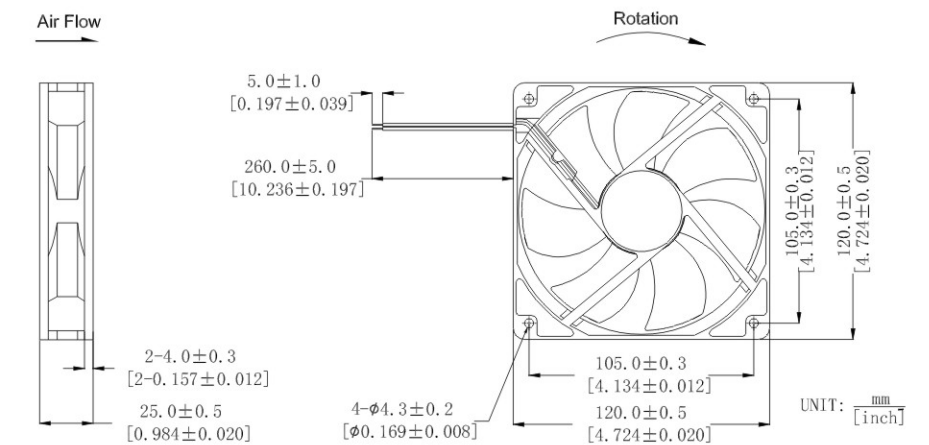
DIMENSIONS DRAWING
