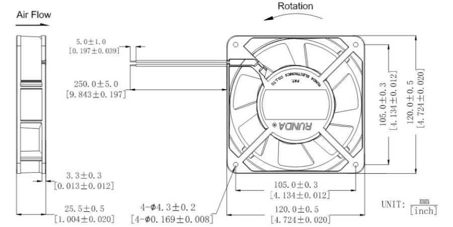
DIMENSIONS DRAWING
