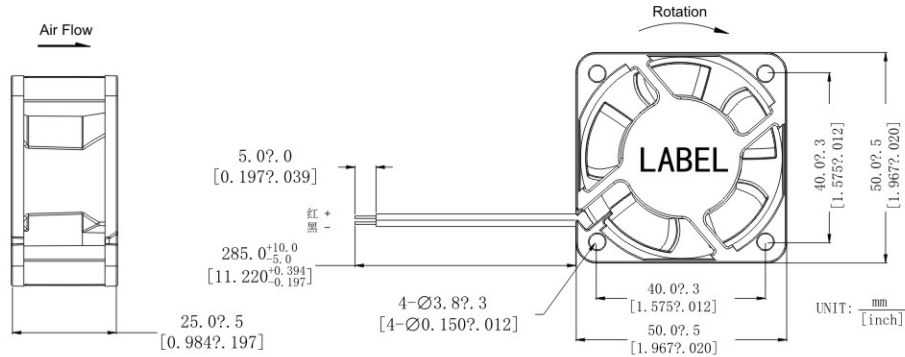
DIMENSIONS DRAWING
