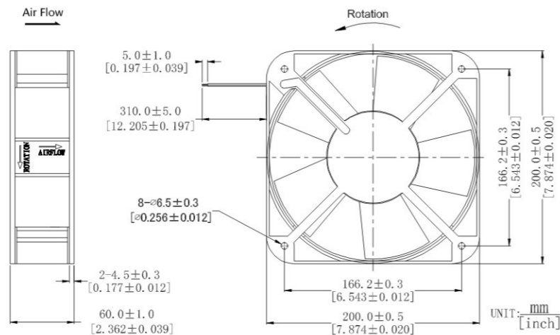
DIMENSIONS DRAWING
