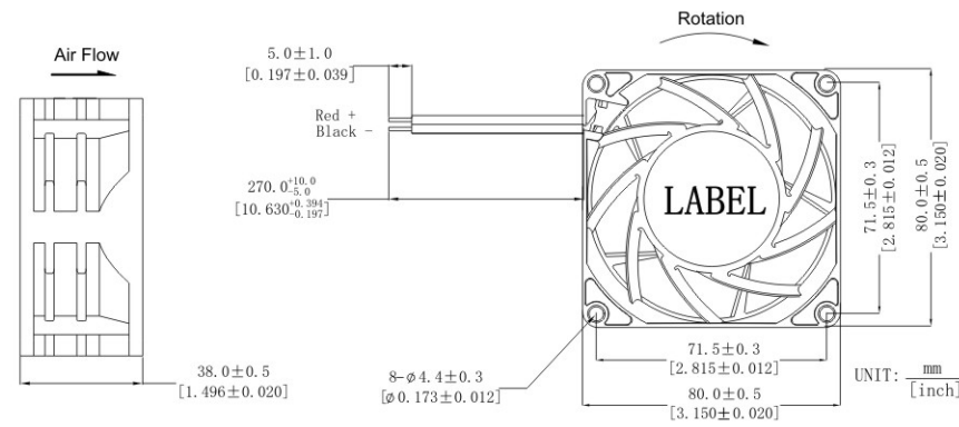
DIMENSIONS DRAWING
