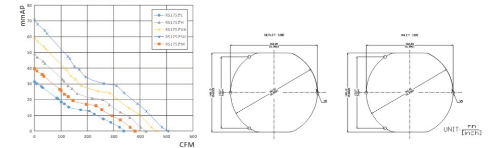
Fan Performance Curve
