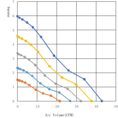
Fan Performance Curve
