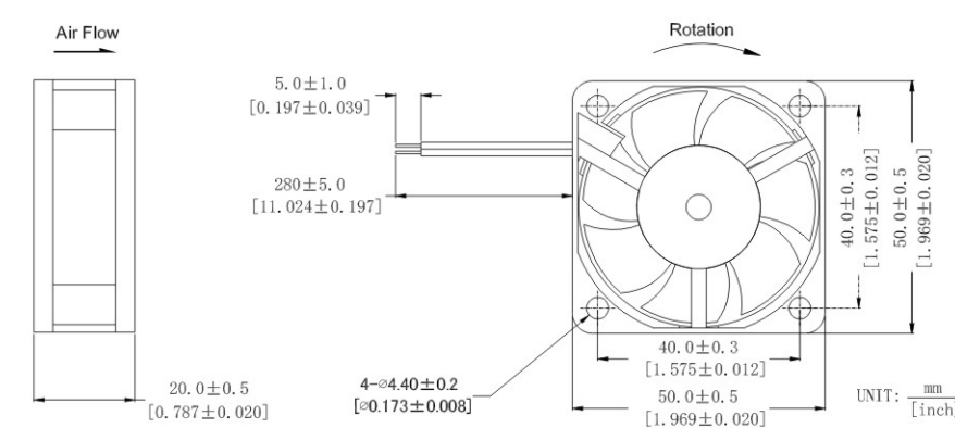
DIMENSIONS DRAWING
