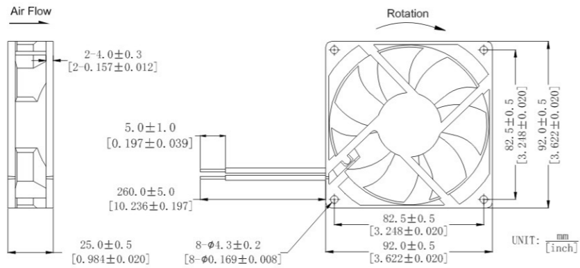
DIMENSIONS DRAWING
