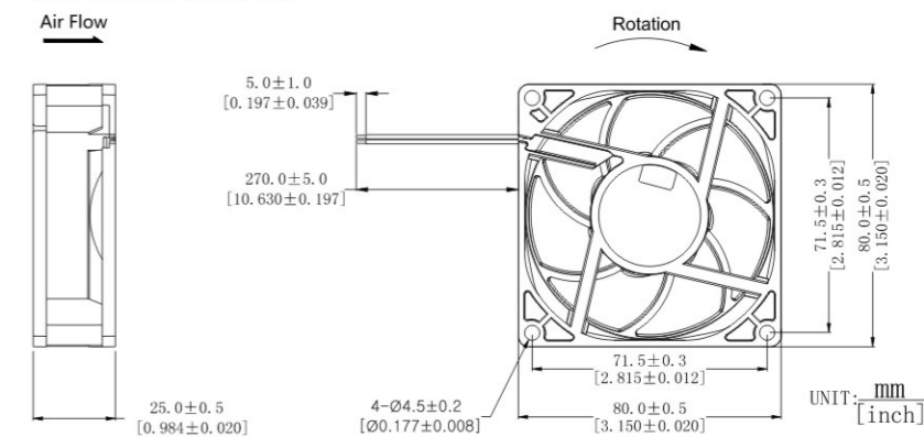
DIMENSIONS DRAWING
