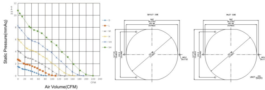
Fan Performance Curve
