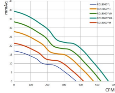
风量风压PQ曲线图 Fan Performance Curve
