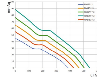
风量风压PQ曲线图 Fan Performance Curve
