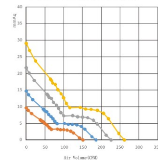
Fan Performance Curve
