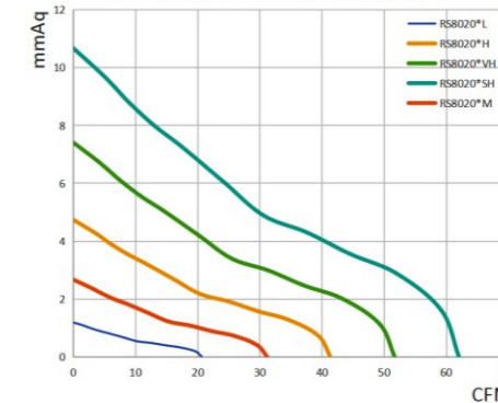
风量风压PQ曲线图 Fan Performance Curve
