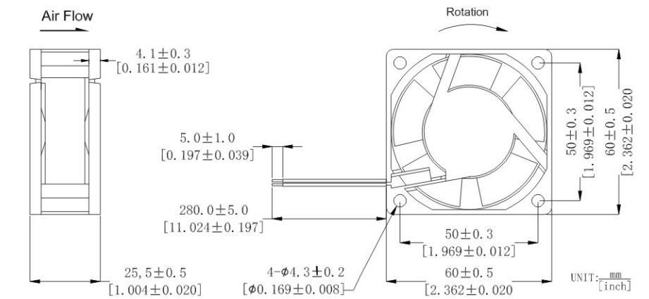
DIMENSIONS DRAWING
