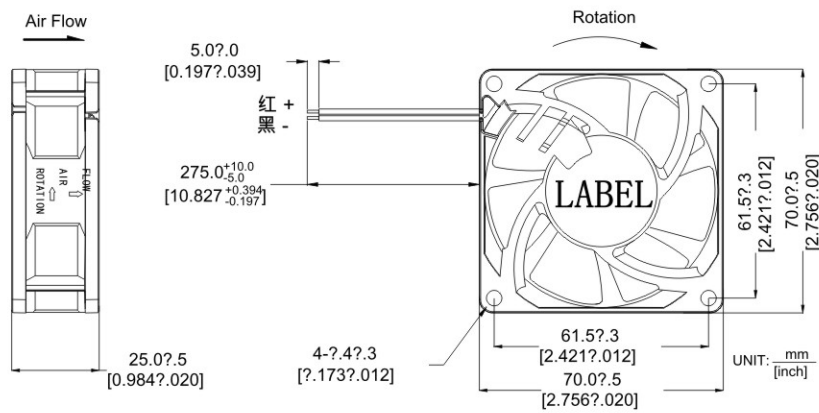
DIMENSIONS DRAWING
