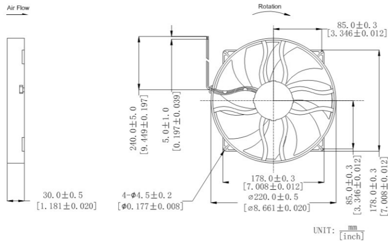
DIMENSIONS DRAWING
