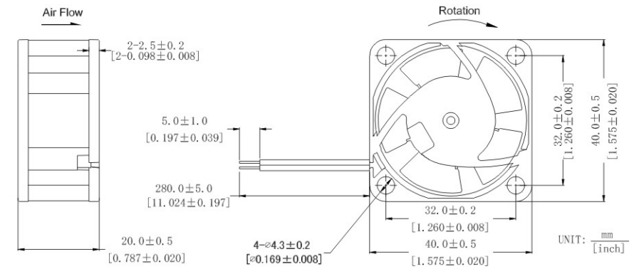
DIMENSIONS DRAWING
