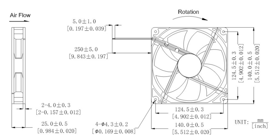
DIMENSIONS DRAWING
