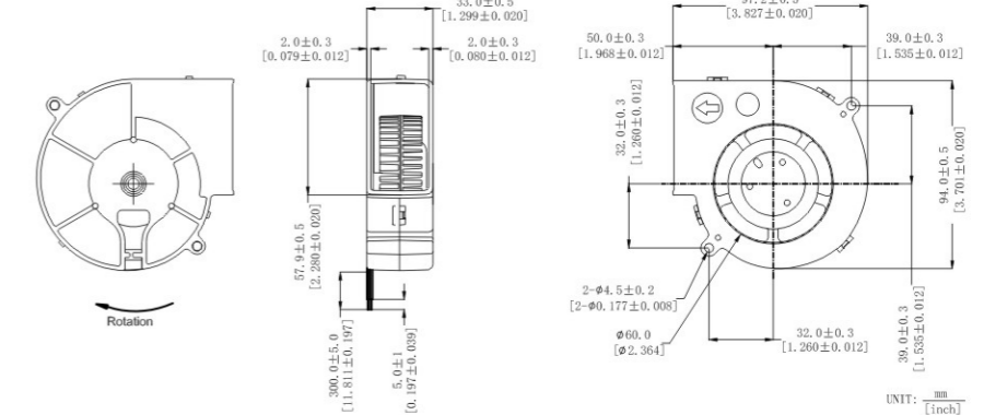
DIMENSIONS DRAWING
