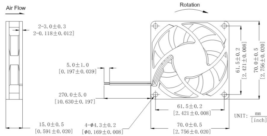
DIMENSIONS DRAWING
