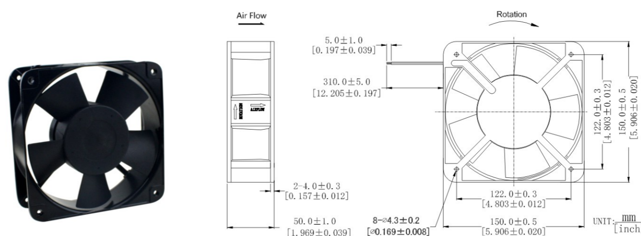
DIMENSIONS DRAWING
