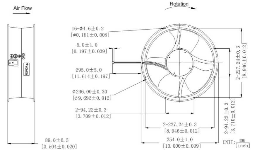
DIMENSIONS DRAWING
