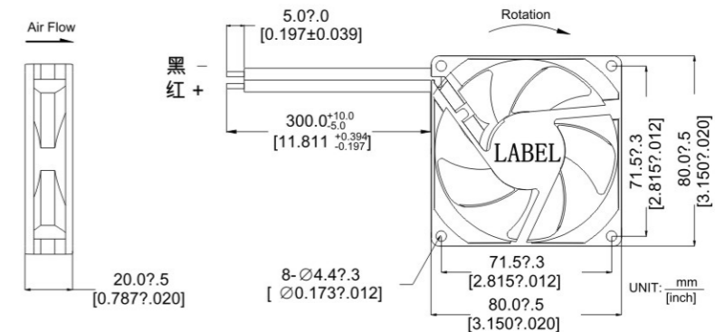
DIMENSIONS DRAWING
