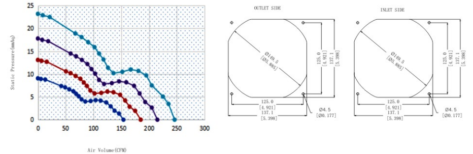
Fan Performance Curve
