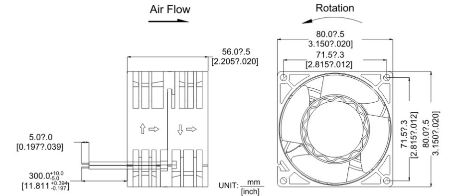
DIMENSIONS DRAWING
