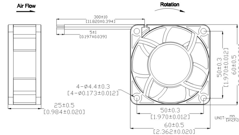
DIMENSIONS DRAWING
