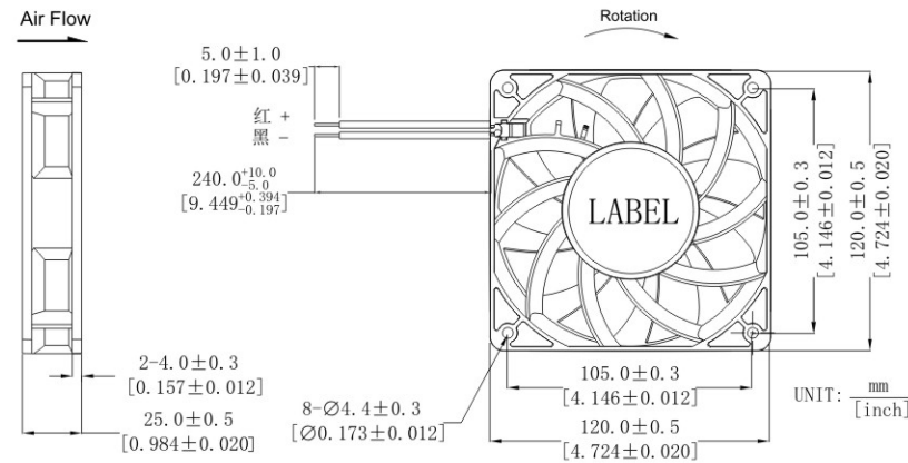
DIMENSIONS DRAWING
