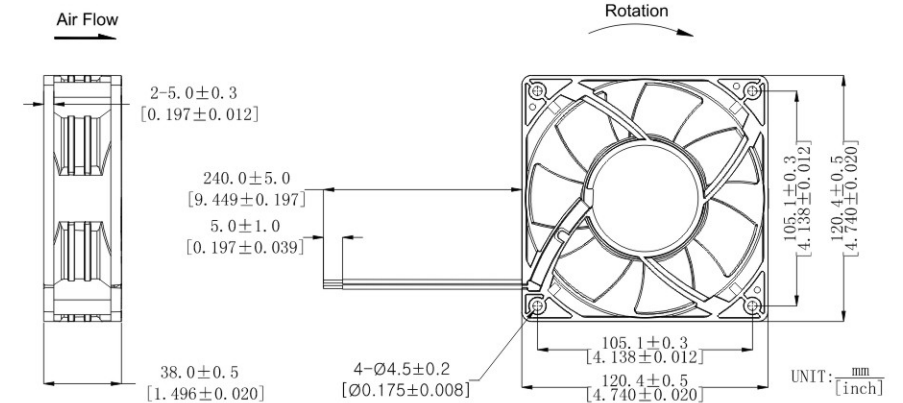
DIMENSIONS DRAWING
