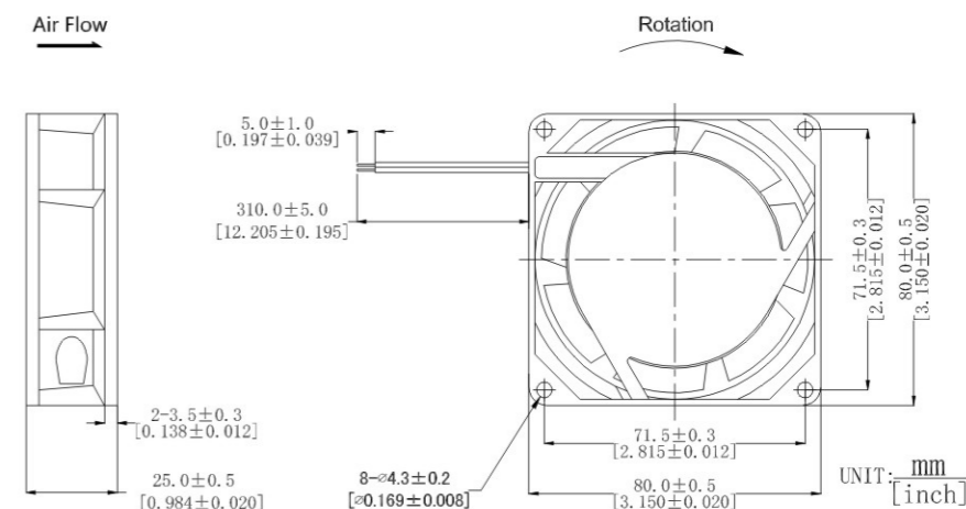
DIMENSIONS DRAWING
