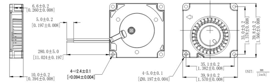
DIMENSIONS DRAWING
