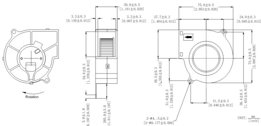
DIMENSIONS DRAWING
