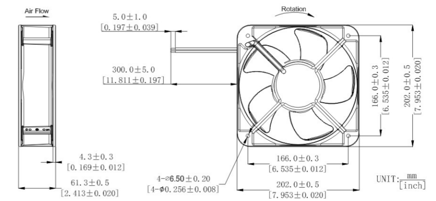
DIMENSIONS DRAWING
