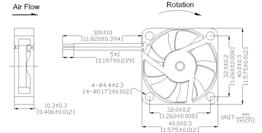
DIMENSIONS DRAWING
