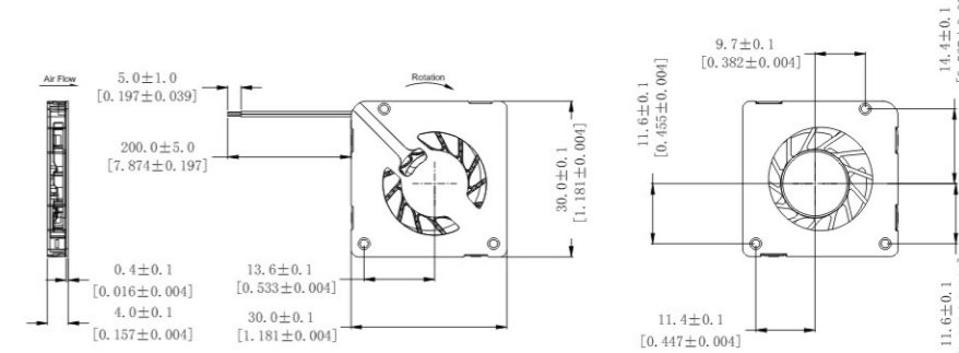
DIMENSIONS DRAWING
