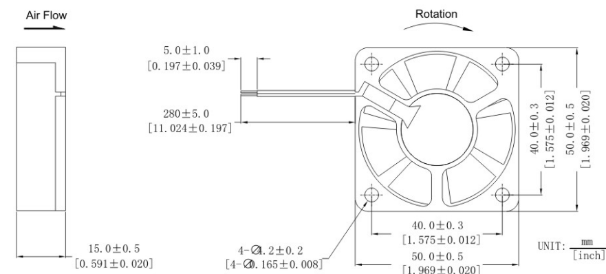
DIMENSIONS DRAWING
