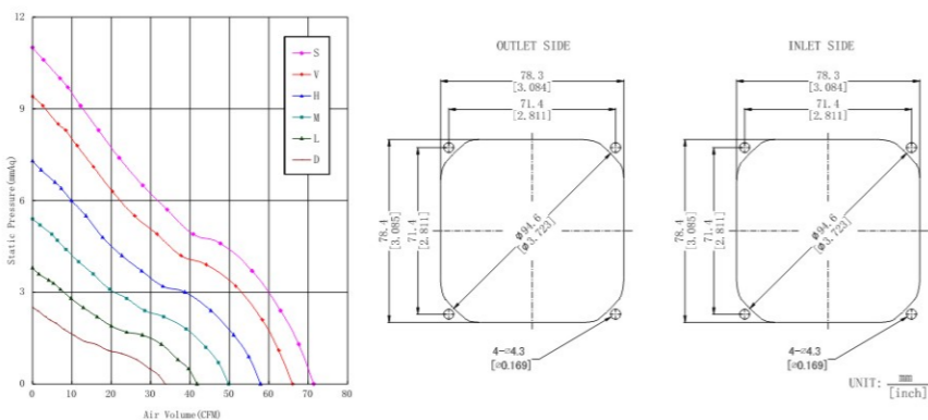
Fan Performance Curve
