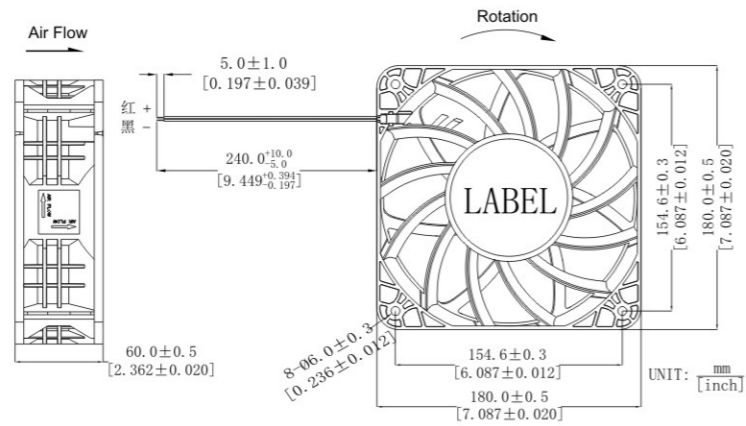
DIMENSIONS DRAWING
