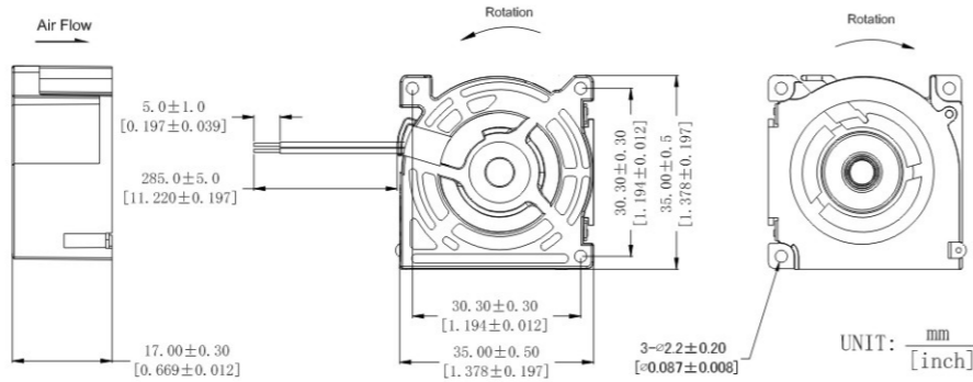
DIMENSIONS DRAWING
