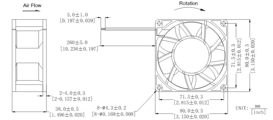
DIMENSIONS DRAWING
