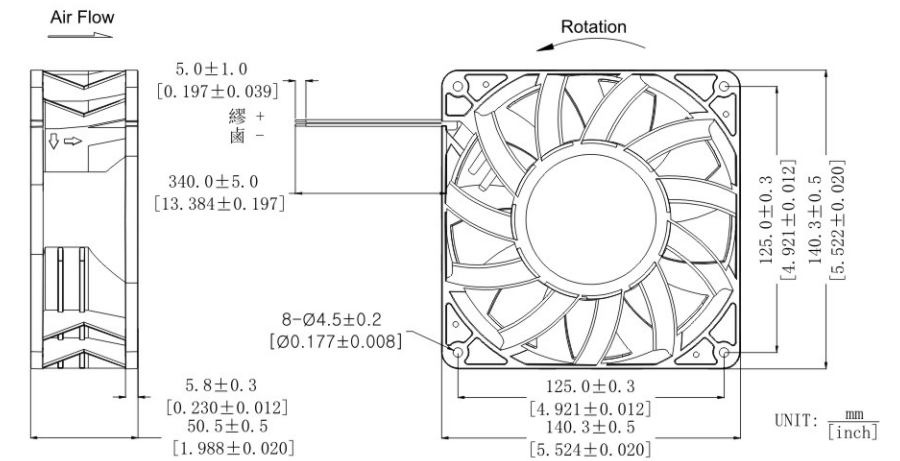
DIMENSIONS DRAWING
