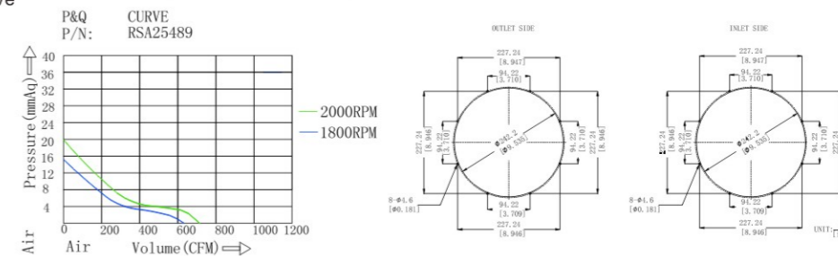
P&Q CURVE (AT RATED VOLTAGE)
