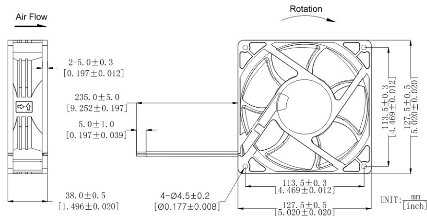
DIMENSIONS DRAWING
