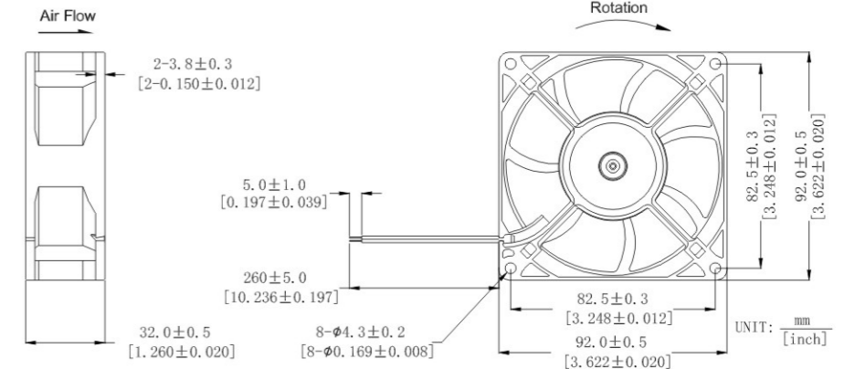
DIMENSIONS DRAWING
