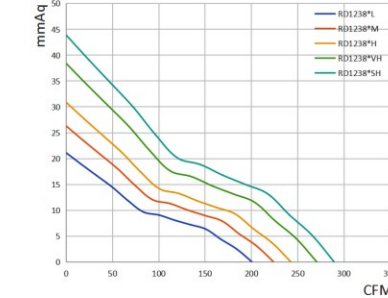
风量风压PQ曲线图 Fan Performance Curve
