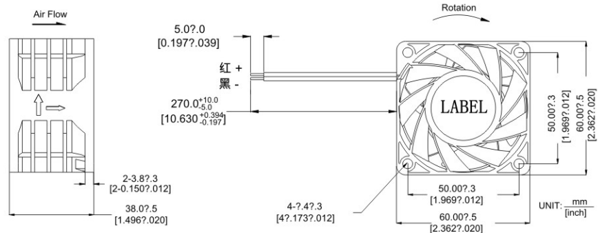
DIMENSIONS DRAWING
