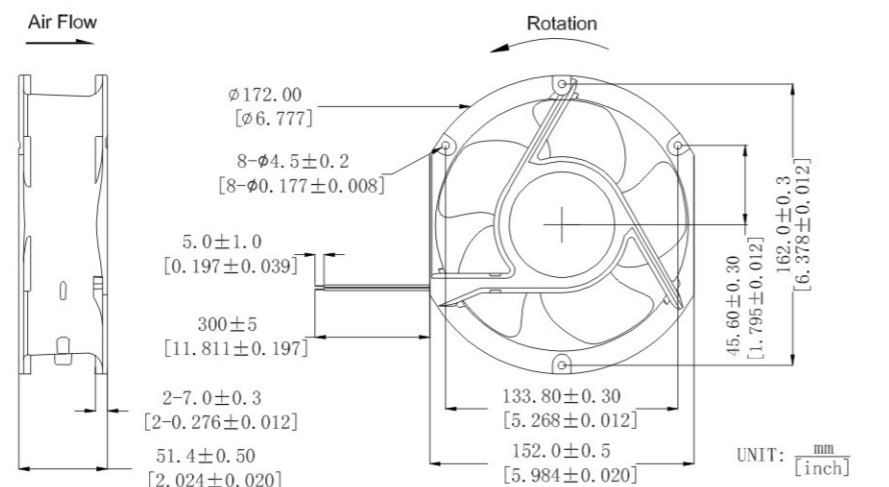
DIMENSIONS DRAWING
