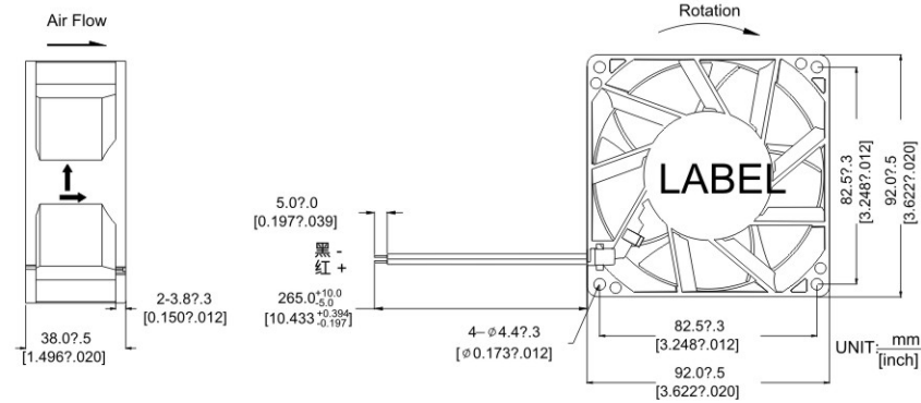
DIMENSIONS DRAWING
