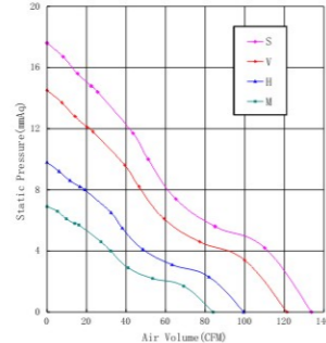
Fan Performance Curve
