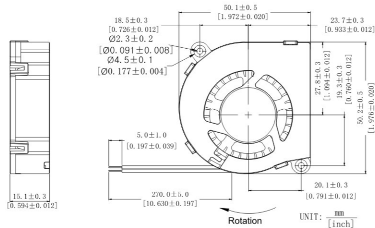
DIMENSIONS DRAWING
