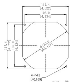
INLET SIDE
