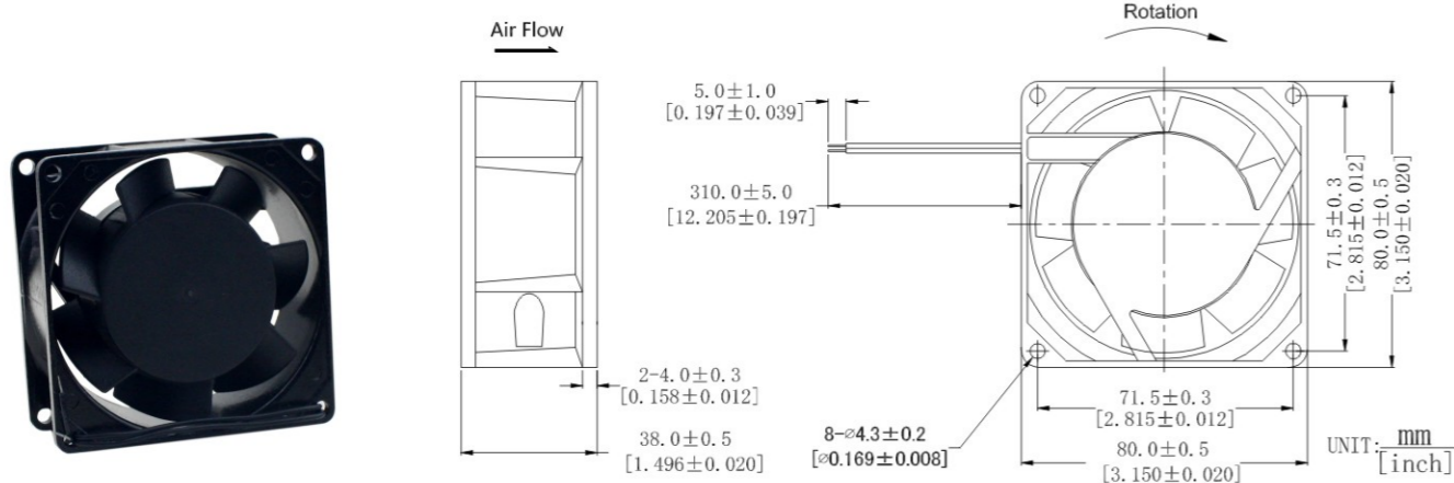
DIMENSIONS DRAWING
