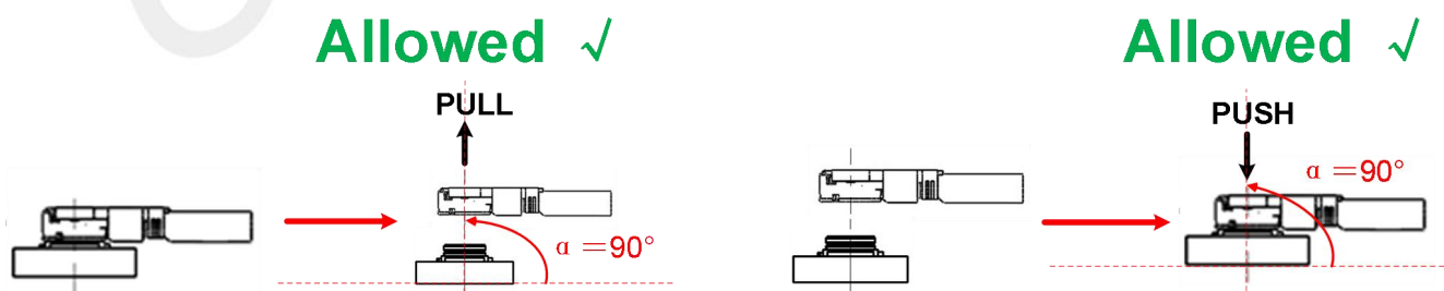
Figure 30: RF cable correct pull and push operation
