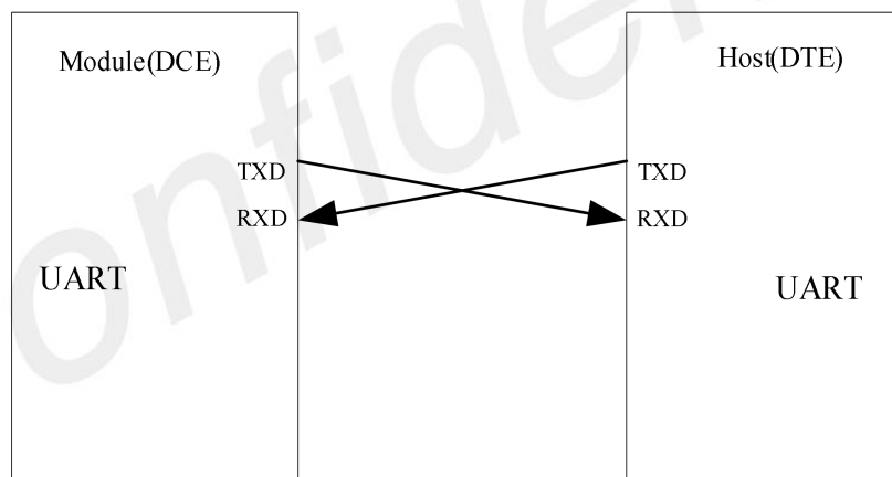
Figure 22: The UART interface reference design
