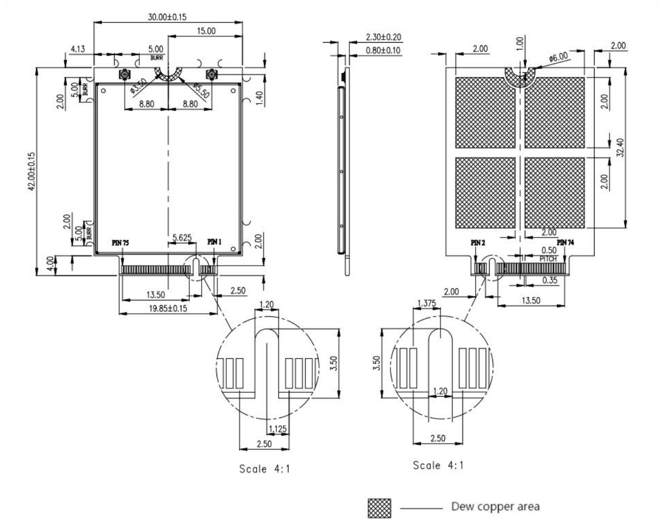
Figure 3: Dimensions of A7908E-M2 (Unit: mm)
