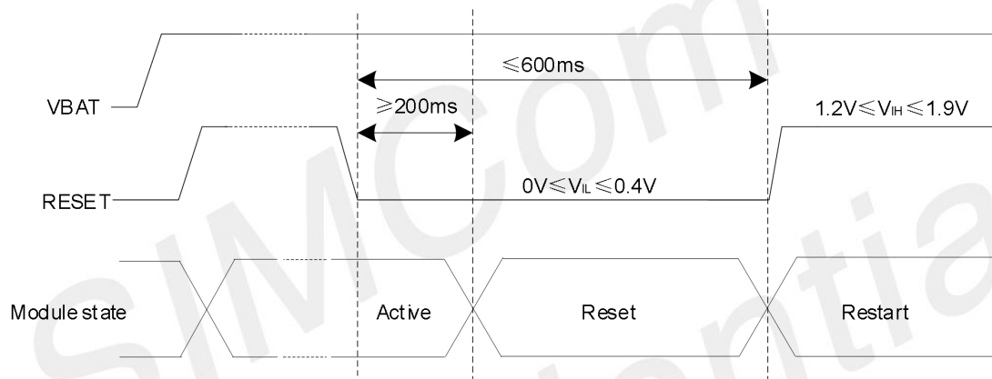
Figure 12: Module reset timing
