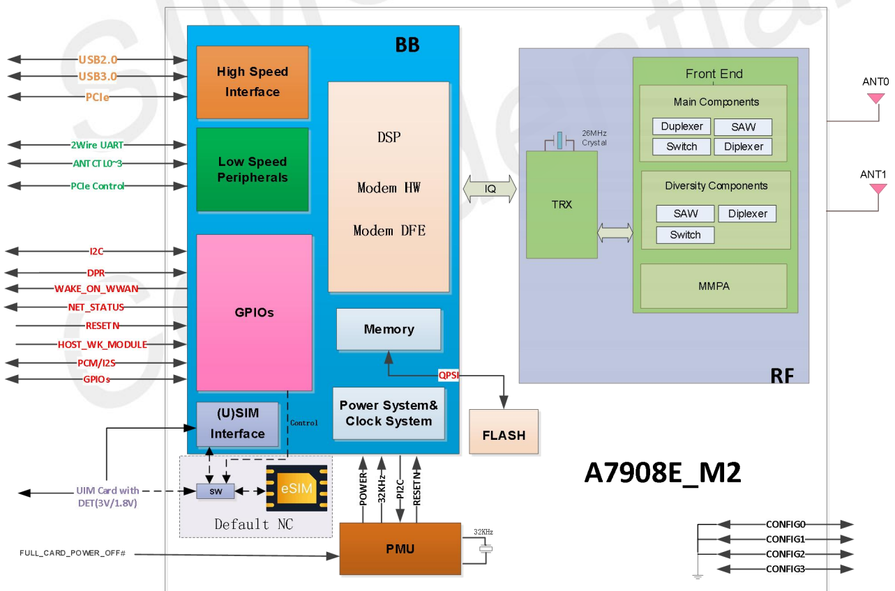
Figure 1: A7908E-M2 block diagram
