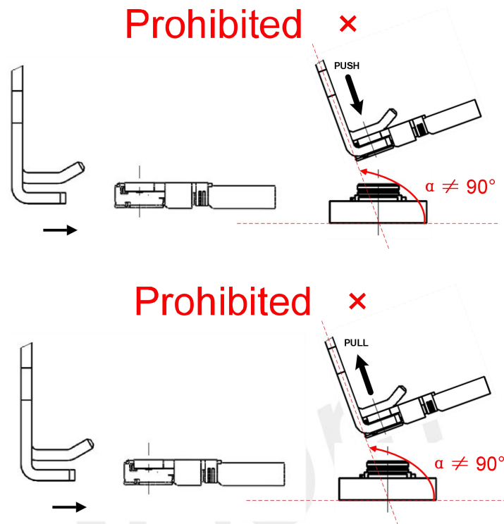
Figure 33: Use RF cable tool error pull and push operation
