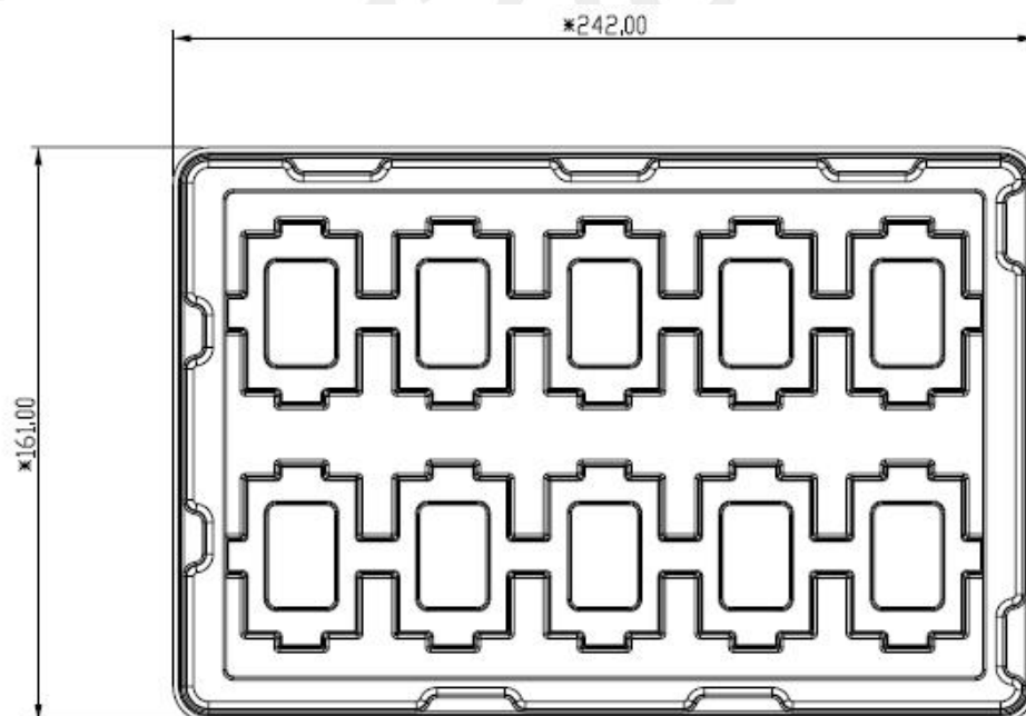
Figure 41: Tray drawing
