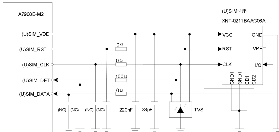
Figure 18: (U)SIM interface reference circuit
