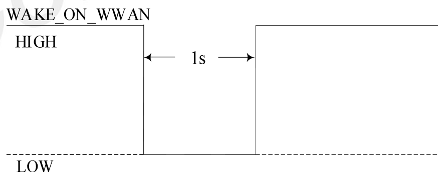
Figure 14: WAKE_ON_WWAN behavior (SMS and URC report etc.)
