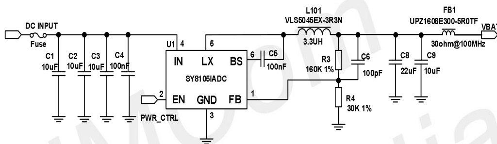
Figure 7: Switch the power supply reference circuit
