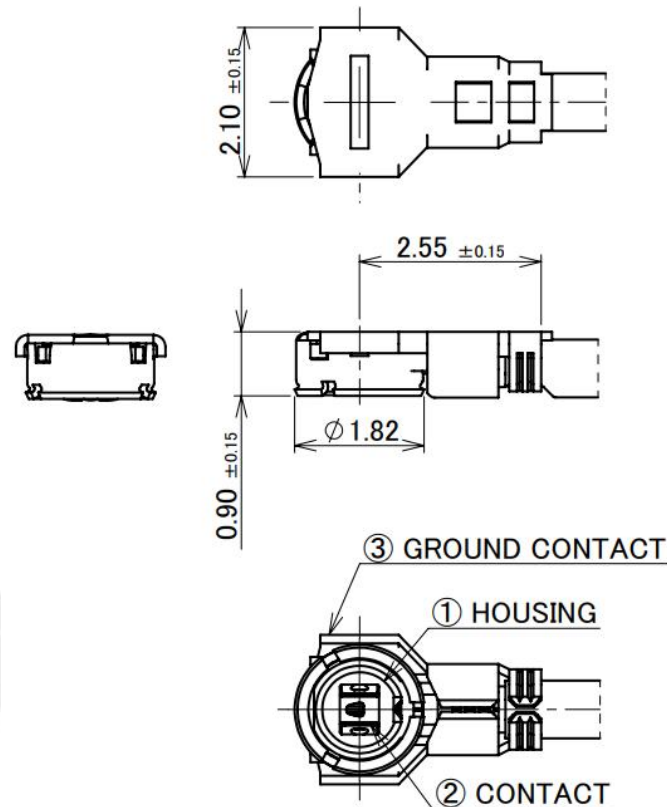
Figure 29: Mechanical information of RF plug
