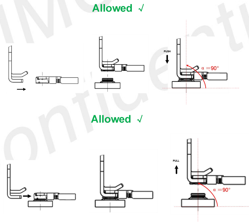
Figure 32: Use RF cable tool correct pull and push operation
