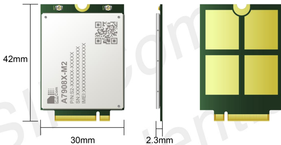
Figure 38: Top and bottom view of module (bottom side reserved ground plane for thermal)
