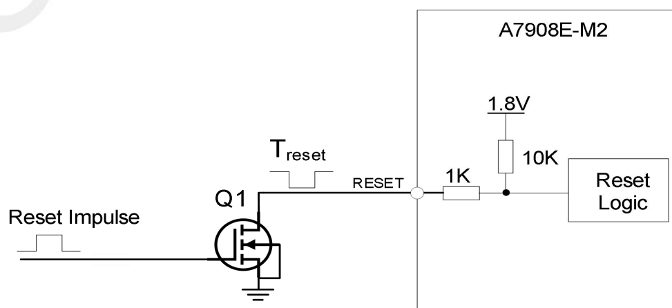
Figure 11: Reference reset circuit
