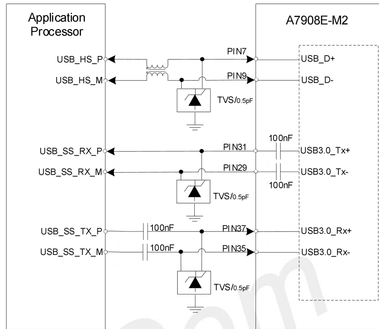
Figure 16: USB reference circuit
