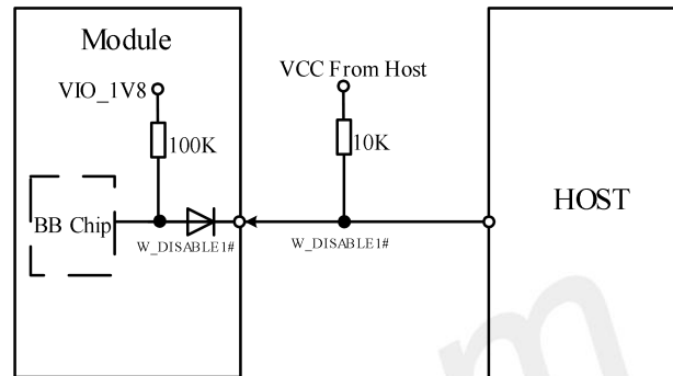
Figure 21: Flight mode switch reference circuit
