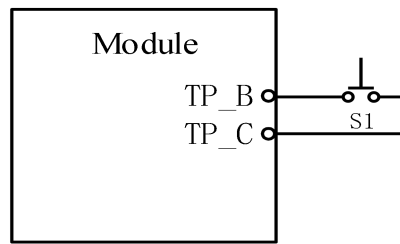
Figure 25: Forcing USB Boot
