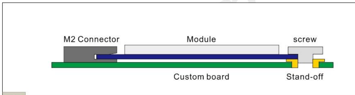
Figure 35:Equipment diagram
