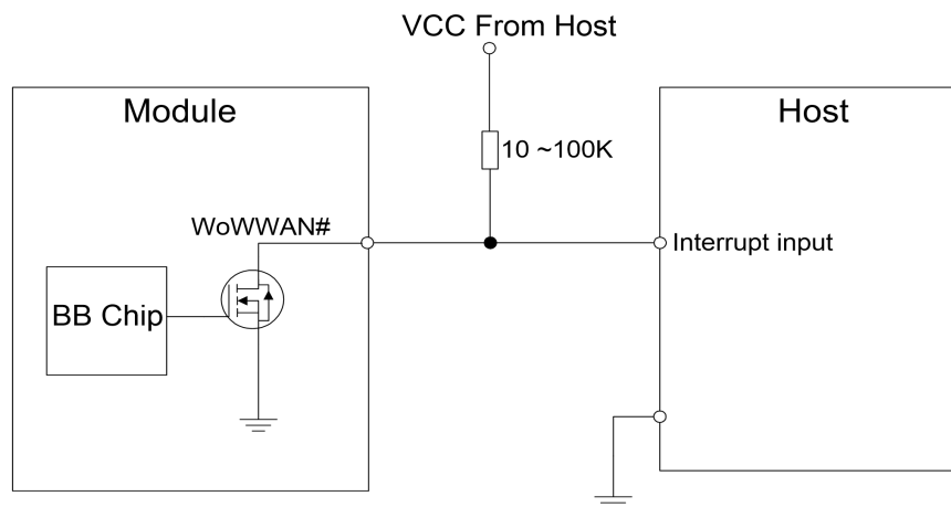
Figure 15: WAKE_ON_WWAN reference circuit
