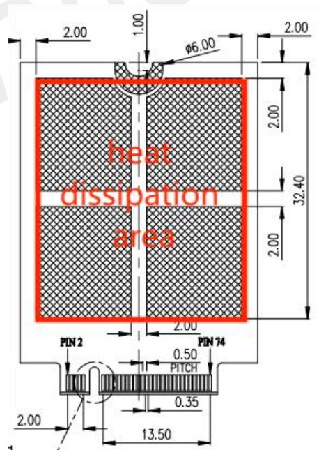
Figure 37: heat dissipation area
