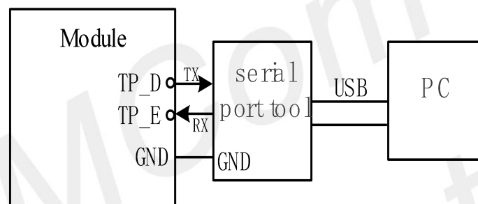
Figure 26: UART LOG
