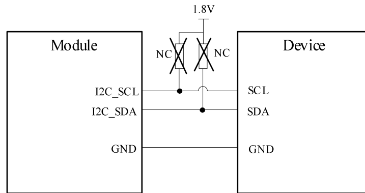
Figure 13: I2C reference circuit
