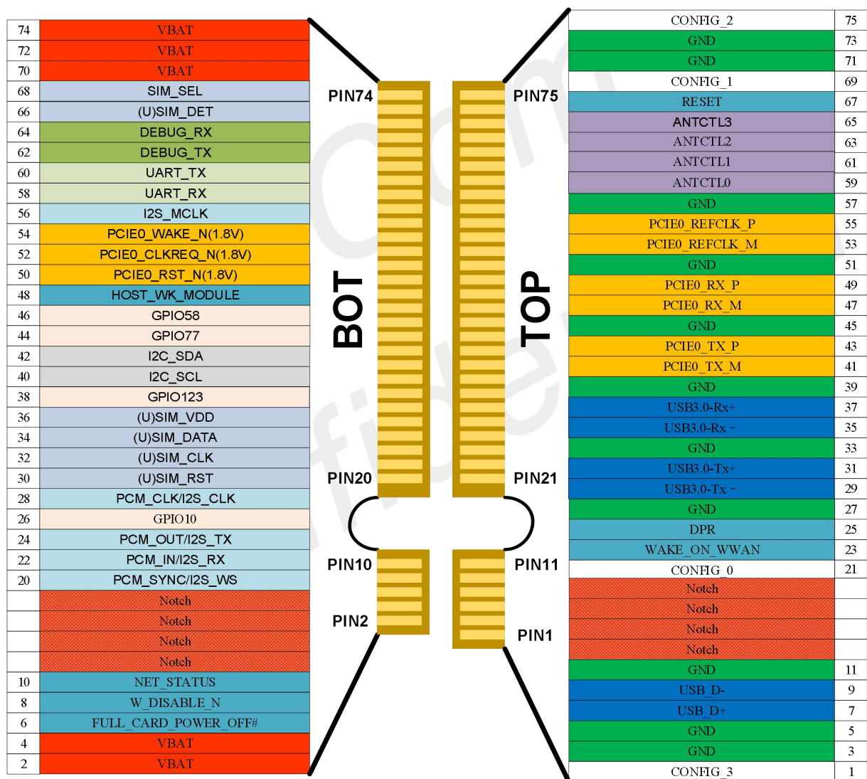
Figure 2: Pin assignment
