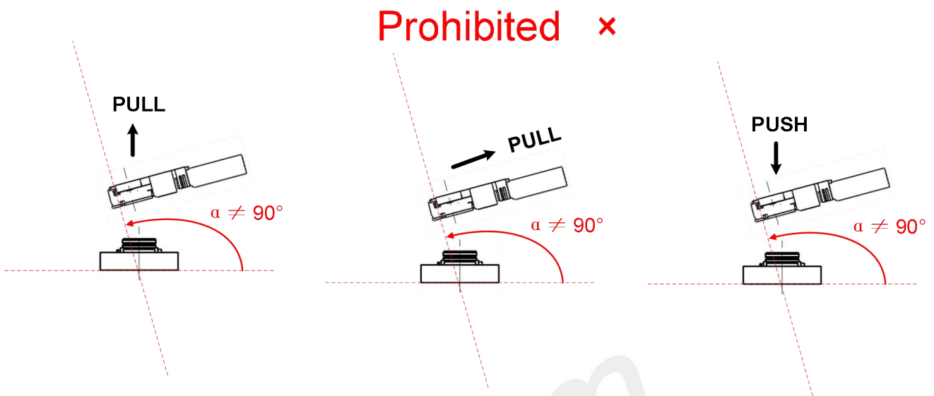
Figure 31: RF cable error pull and push operation
