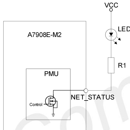
Figure 20: NET_STATUS reference circuit
