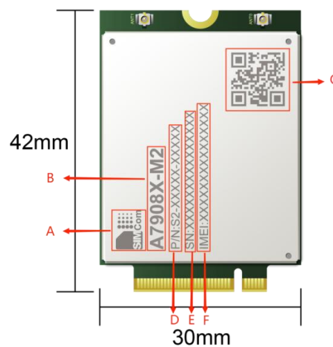
Figure 39: Label information
