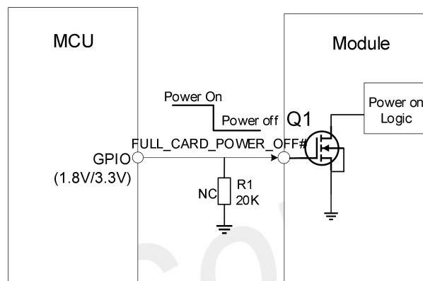
Figure 8: Reference power on/off circuit
