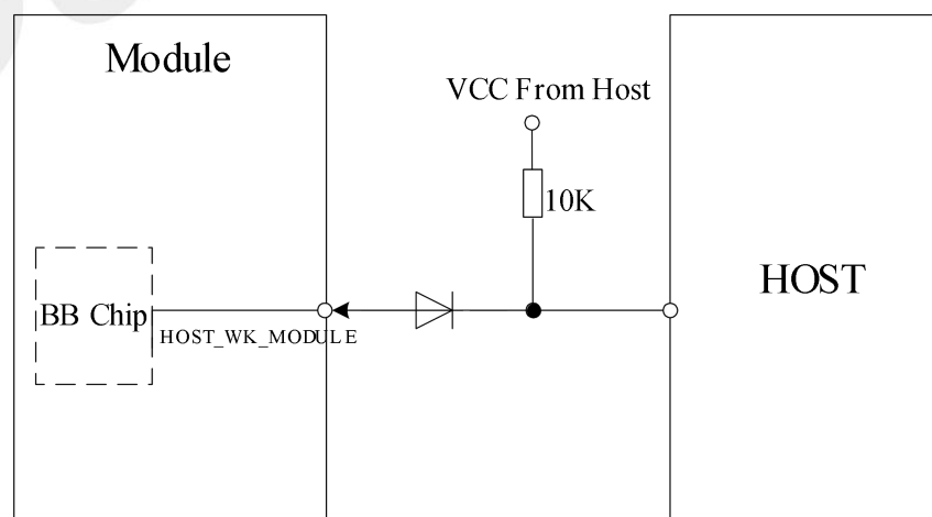
Figure 27: HOST_WK_MODULE interface recommended reference circuit
