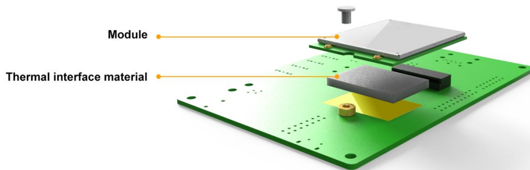
Figure 36: Thermal design
