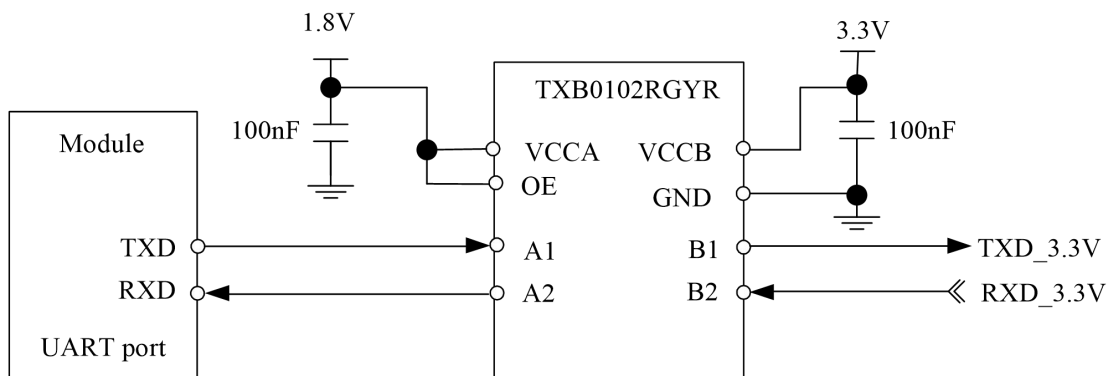
Figure 23: Reference circuit of level shift
