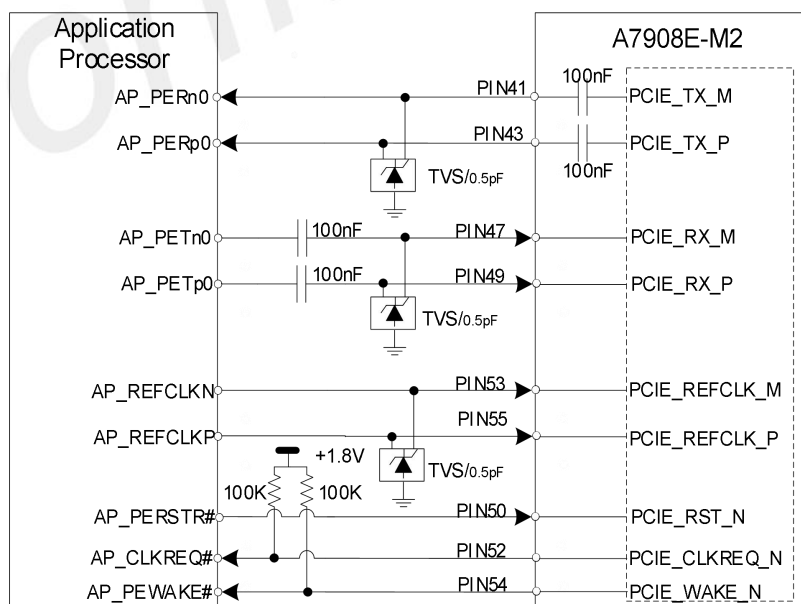
Figure 17: PCIe interface reference circuit
