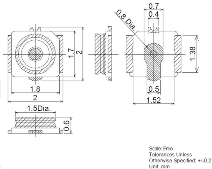
Figure 28: RF connector
