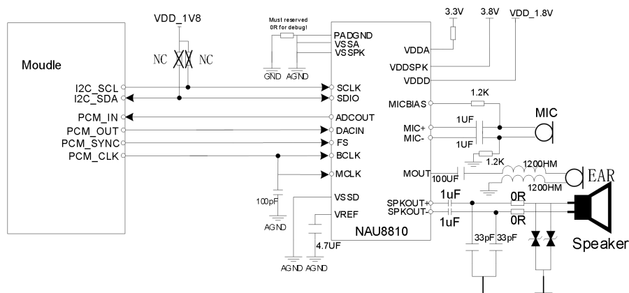
Figure 19: Audio codec diagram circuit
