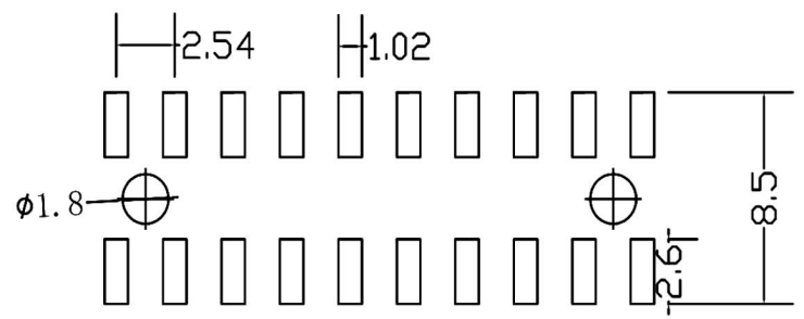
PCB LAYOUT
