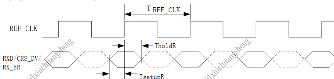
Figure 5-41. RMII Receive Timing
