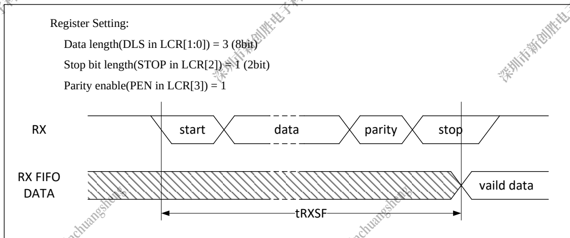
Figure 5-48. UART RX Timing
