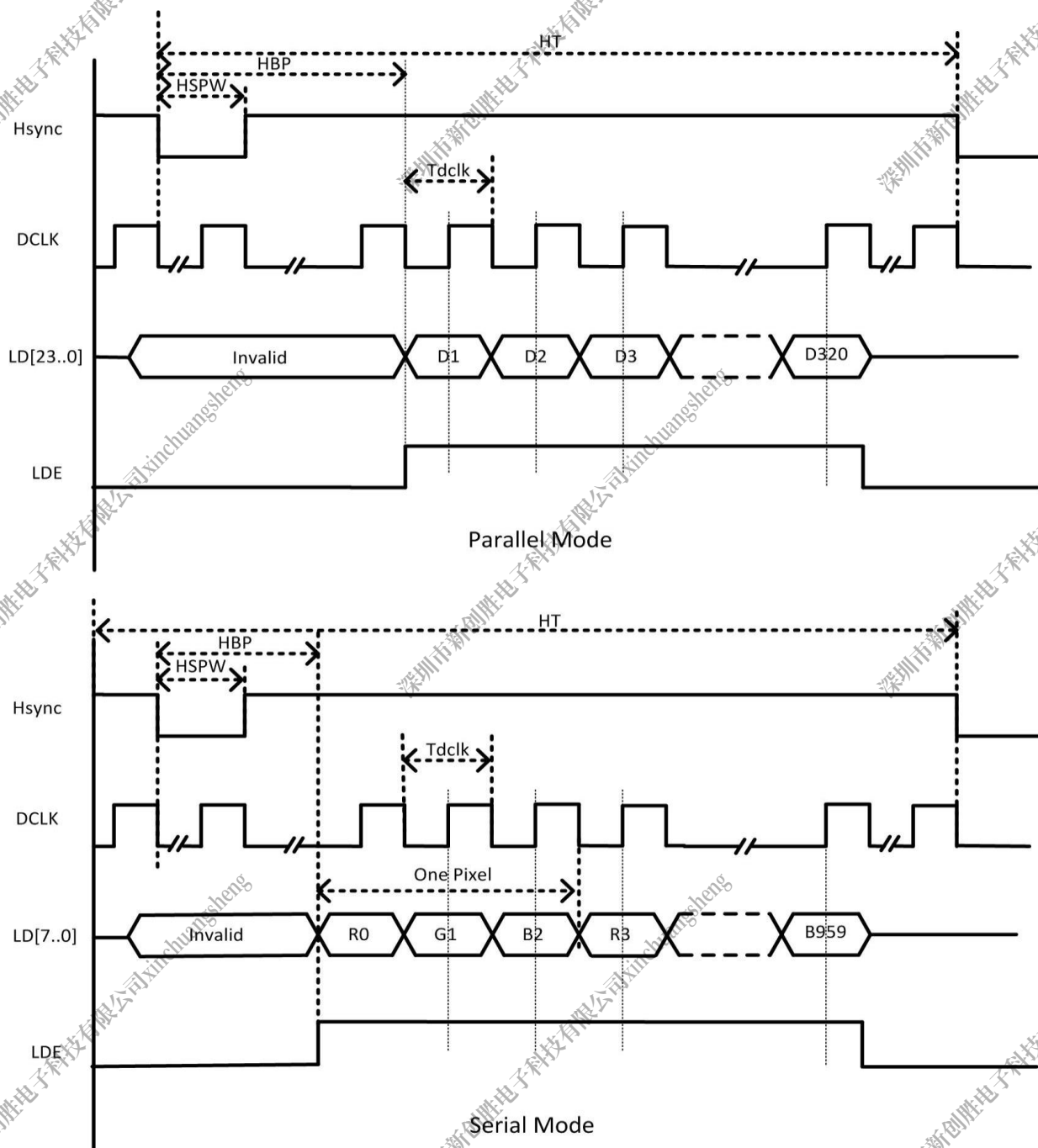
Figure 5-39. HV_IF Interface Horizontal Timing
