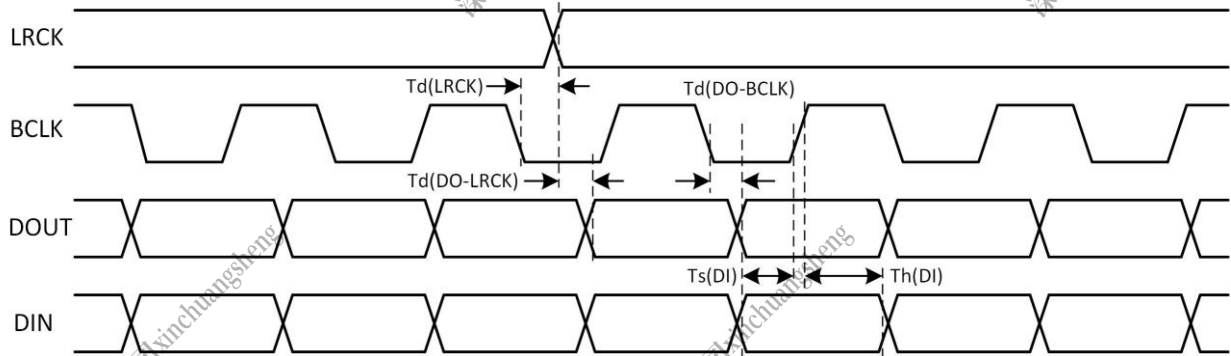
Figure 5-53. I2S/PCM Timing in Master Mode
