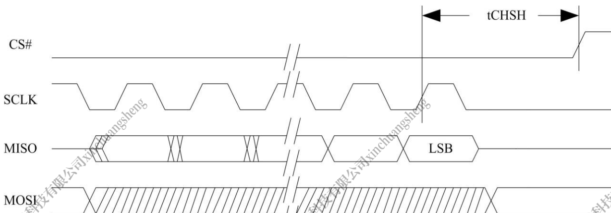
Figure 5-47. SPI MISO Timing
