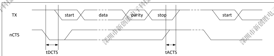
Figure 5-49. UART nCTS Timing
