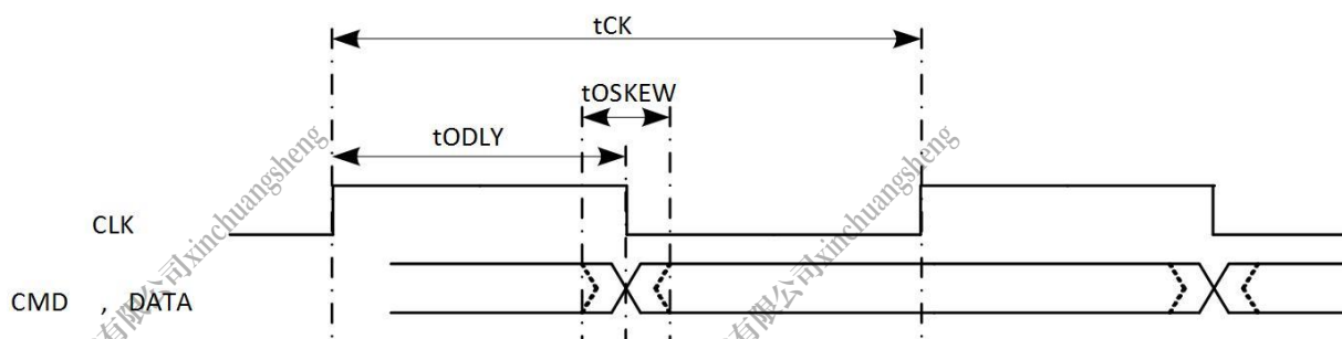
Figure 5-34. SMHC2 HS200 Mode Output Timing Diagram
