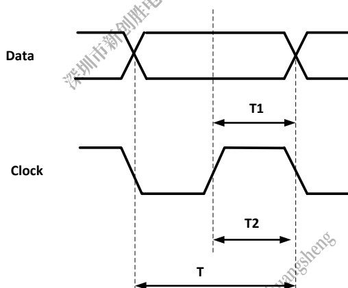
Figure 5-52. TSC Data and Clock Timing
