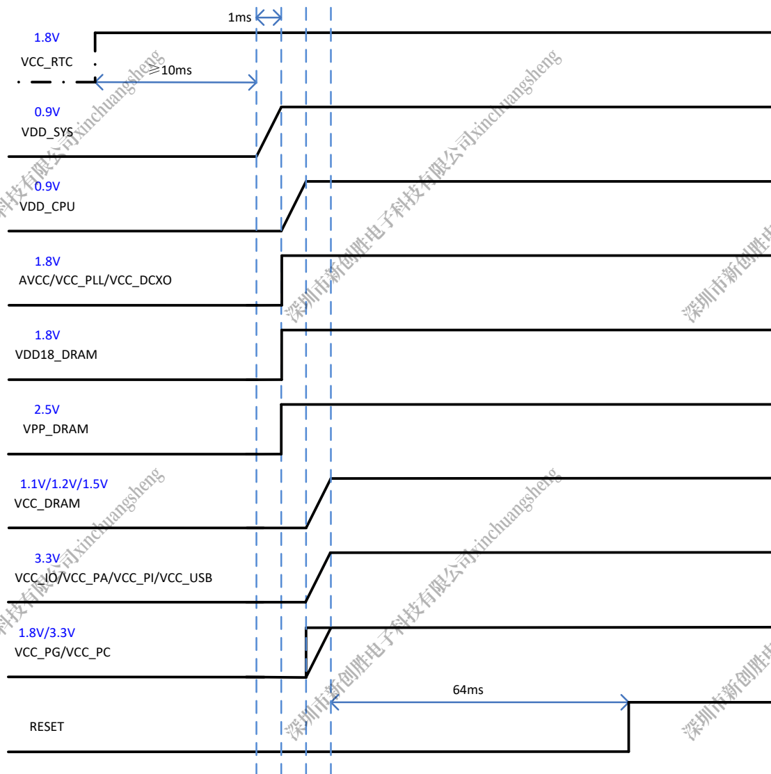
Figure 5-57. Power On Timing
