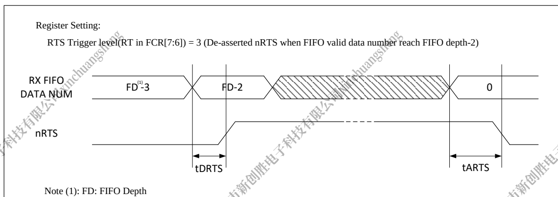
Figure 5-50. UART nRTS Timing
