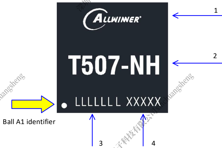
Figure 11-3 T507-NH Marking
