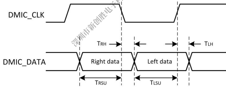
Figure 5-55. DMIC Timing
