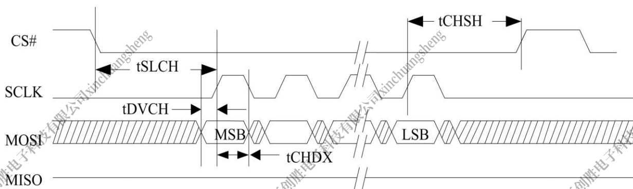
Figure 5-46. SPI MOSI Timing
