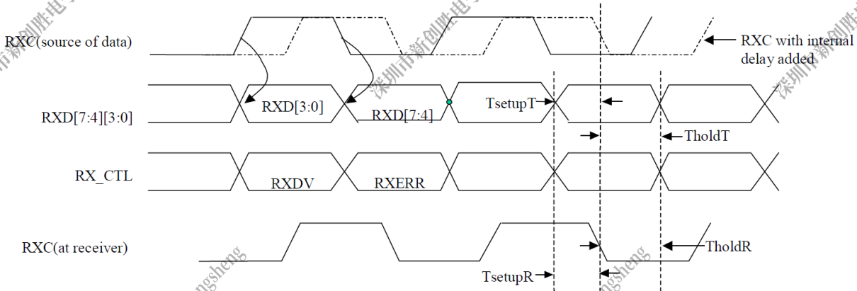
Figure 5-43. RGMII Receive Timing
