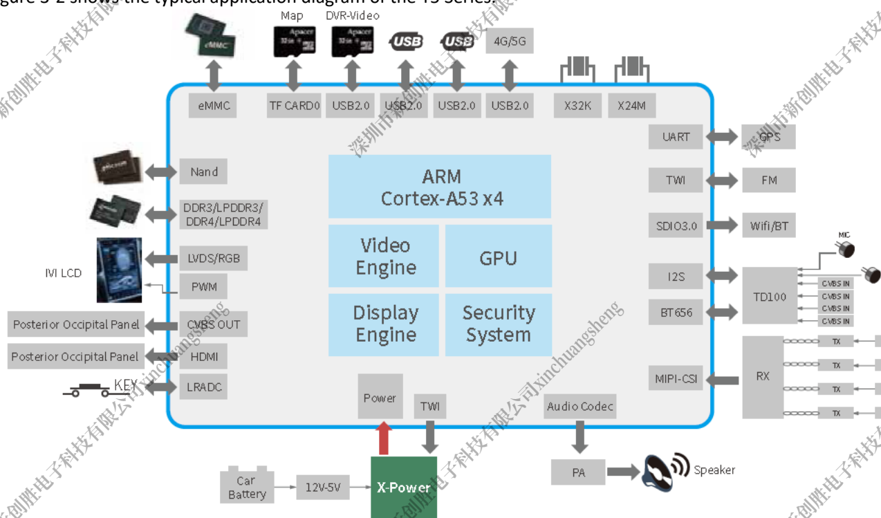
Figure 3-2 shows the typical application diagram of the T5 Series
