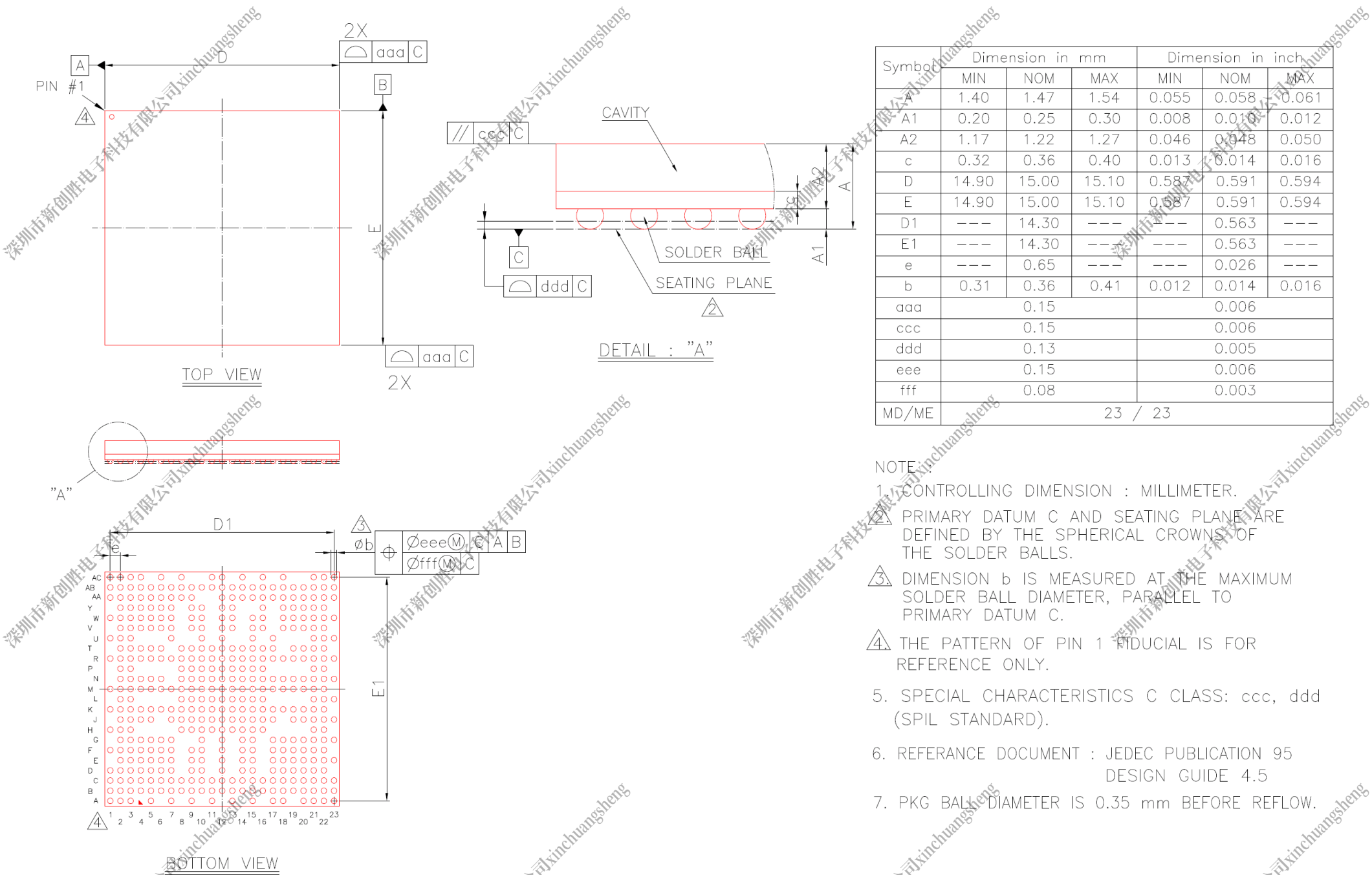
Figure 7-3. T5 Series Package Dimension
