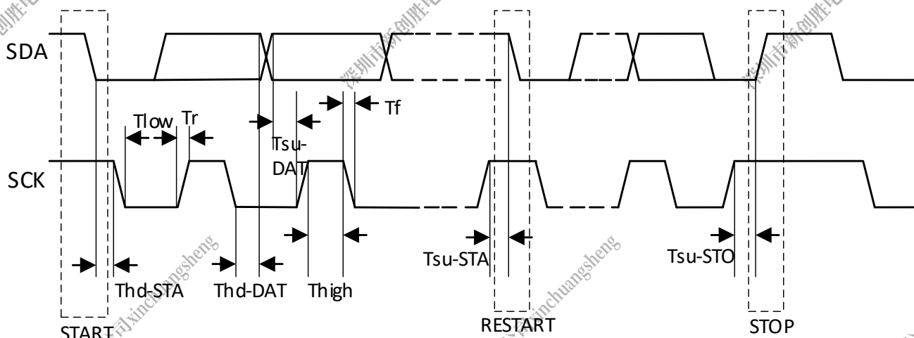
Figure 5-51. TWI Timing
