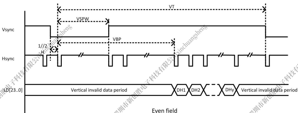
Figure 5-38. HV_IF Interface Vertical Timing
