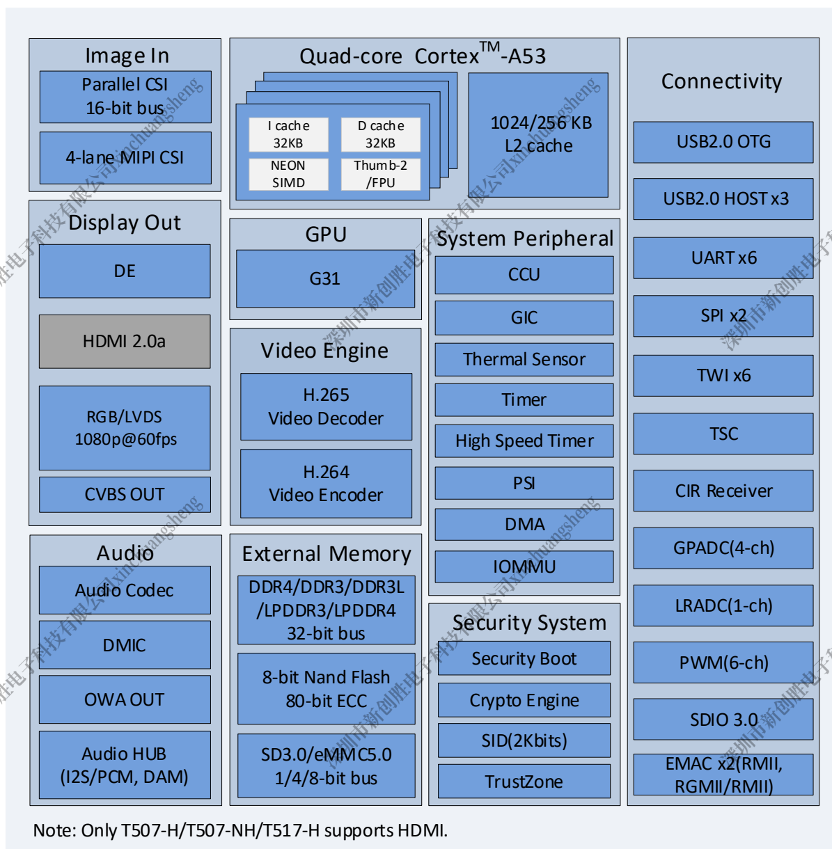
Figure 3-1. T5 Series System Block Diagram
