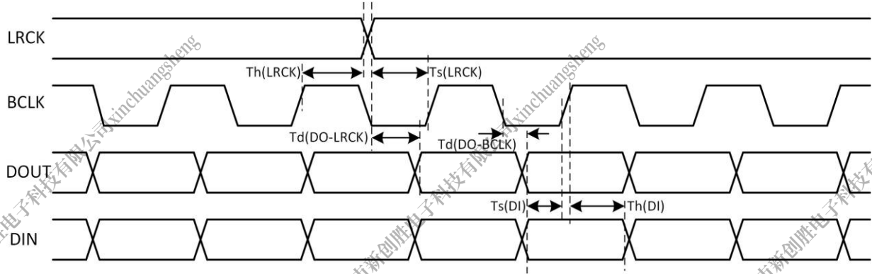
Figure 5-54. I2S/PCM Timing in Slave Mode
