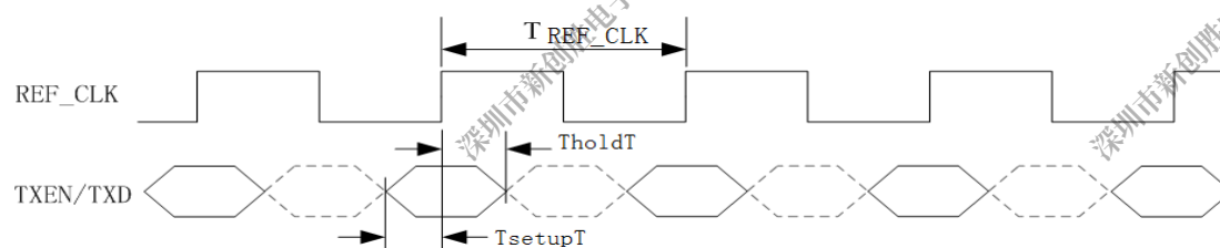
Figure 5-42. RMII Transmit Timing
