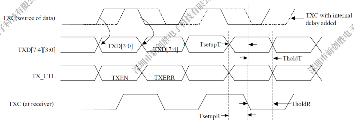
Figure 5-44. RGMII Transmit Timing
