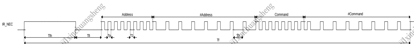
Figure 5-45. CIR-RX Timing
