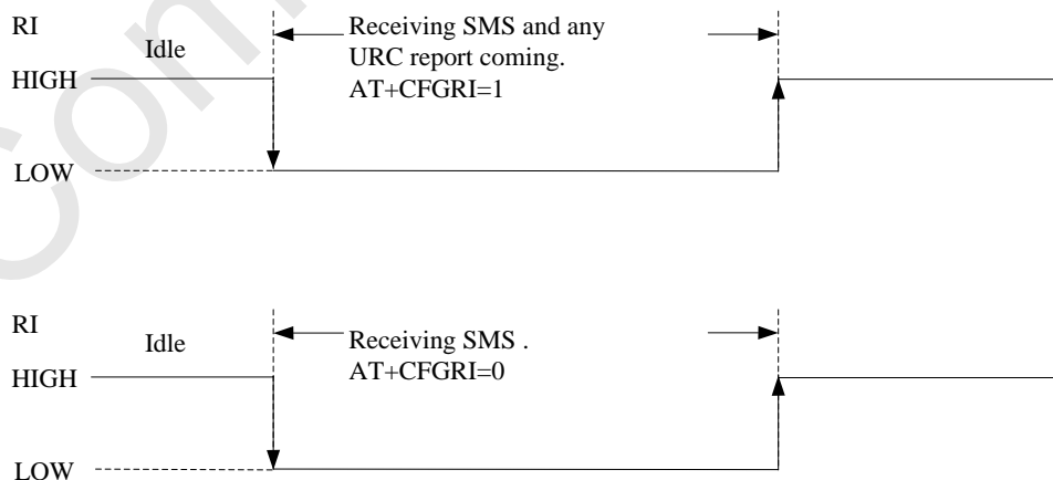
Figure 17: RI behaviour (SMS and URC report)
