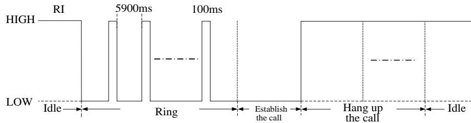
Figure 18: RI behaviour (voice call)
