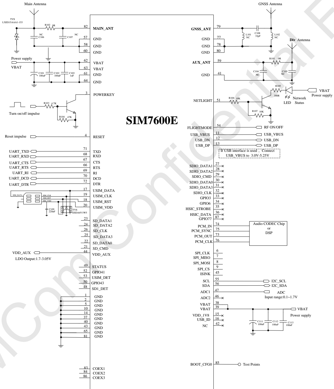
Figure 41: Reference design
