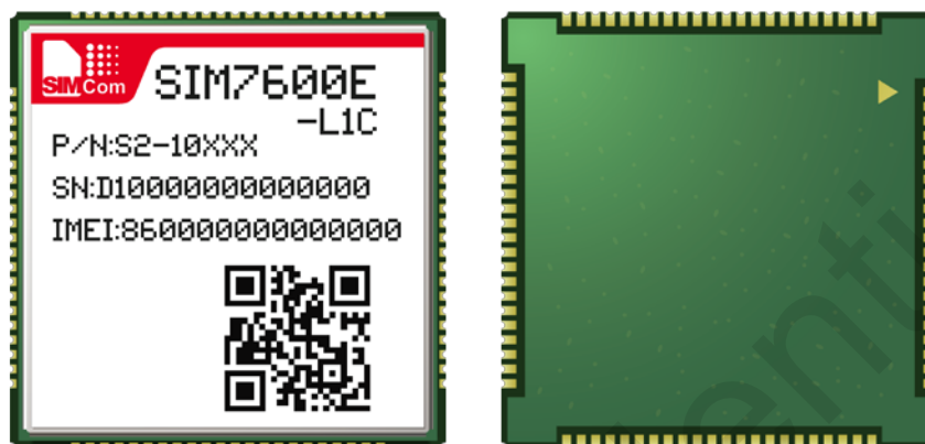
Figure 34: Top and bottom view of module
