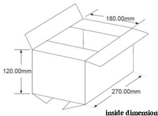
Figure 39: Small carton drawing
