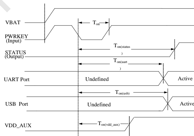
Figure 10: Power on timing sequence
