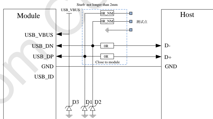
Figure 19: USB reference circuit
