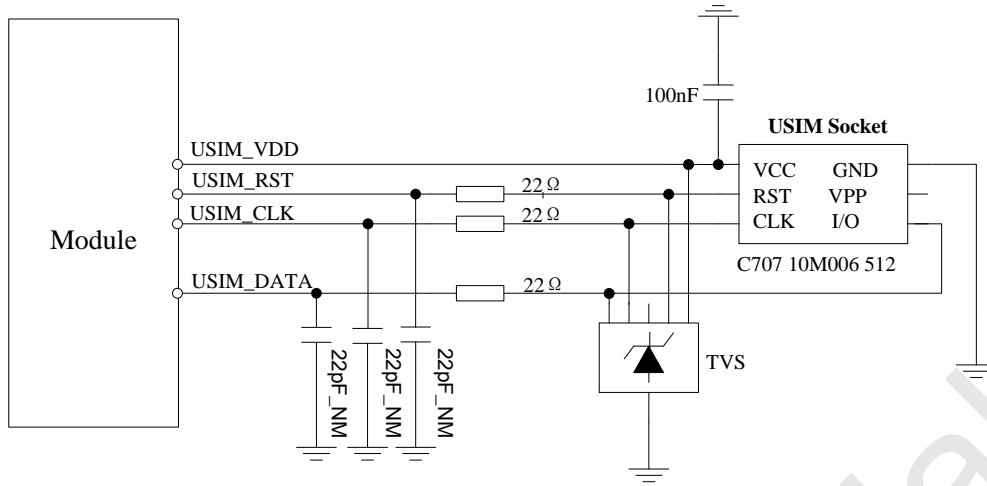
Figure 20: USIM interface reference circuit
