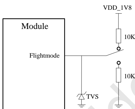
Figure 29: Flight mode switch reference circuit
