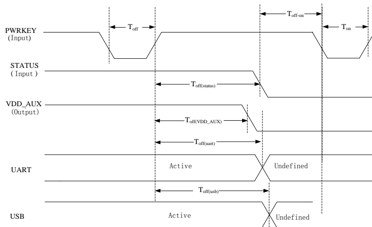
Figure 11: Power off timing sequence
