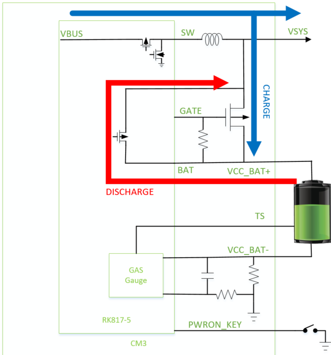
Figure 4: Power With Battery
