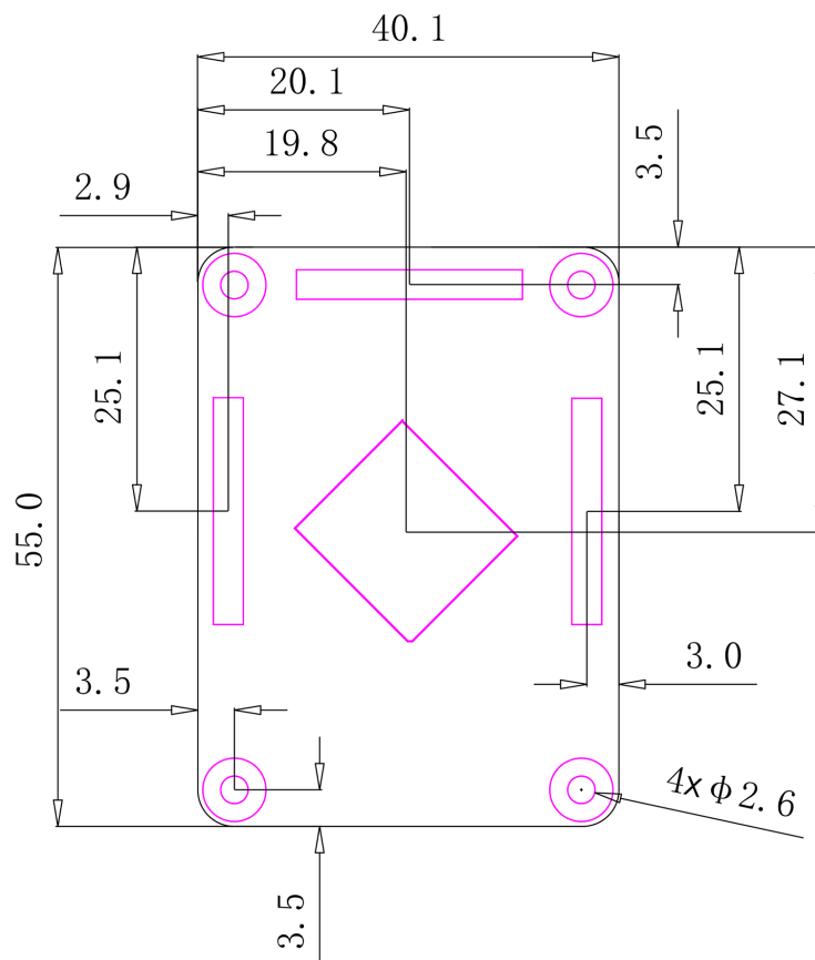
Figure 13: Radxa CM3 Dimensions
