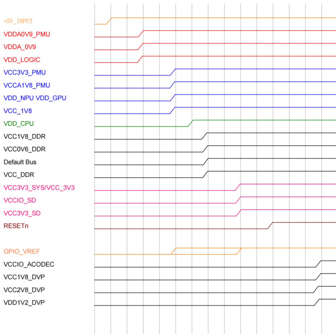
Figure 3: Power On Sequence with +5V_INPUT
