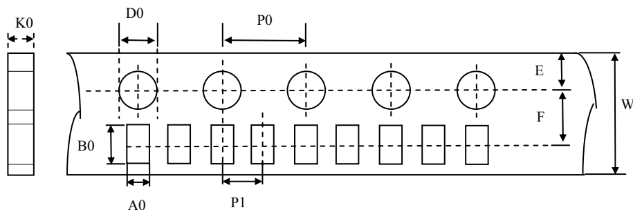
Carrier tape dimensions. (Unit: mm)
