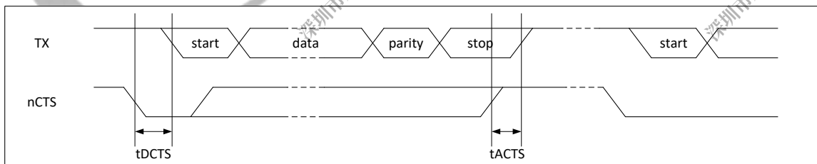
Figure 4-36 UART nCTS Timing
