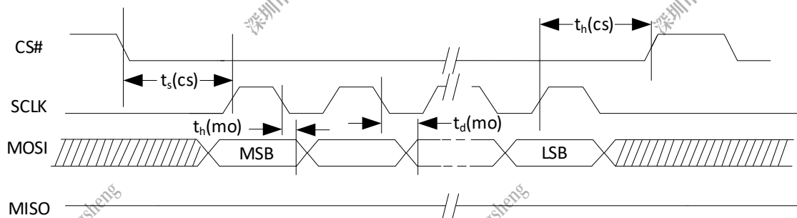
Figure 4-29 SPI Writing Timing
