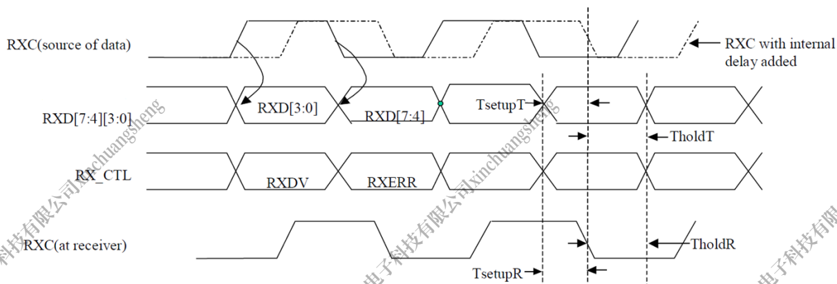
Figure 4-26 RGMII Transmit Timing
