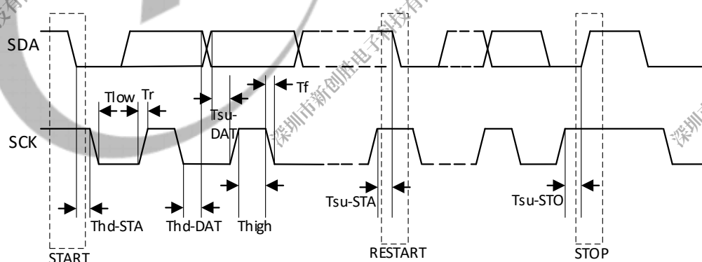
Figure 4-38 TWI Timing
