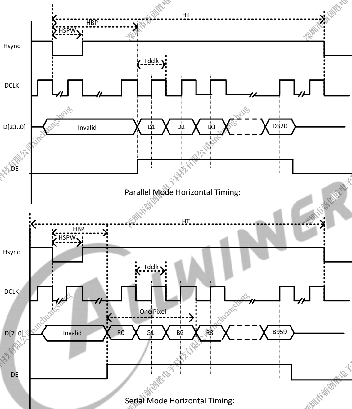
Figure 4-21 HV_IF Horizontal Timing
