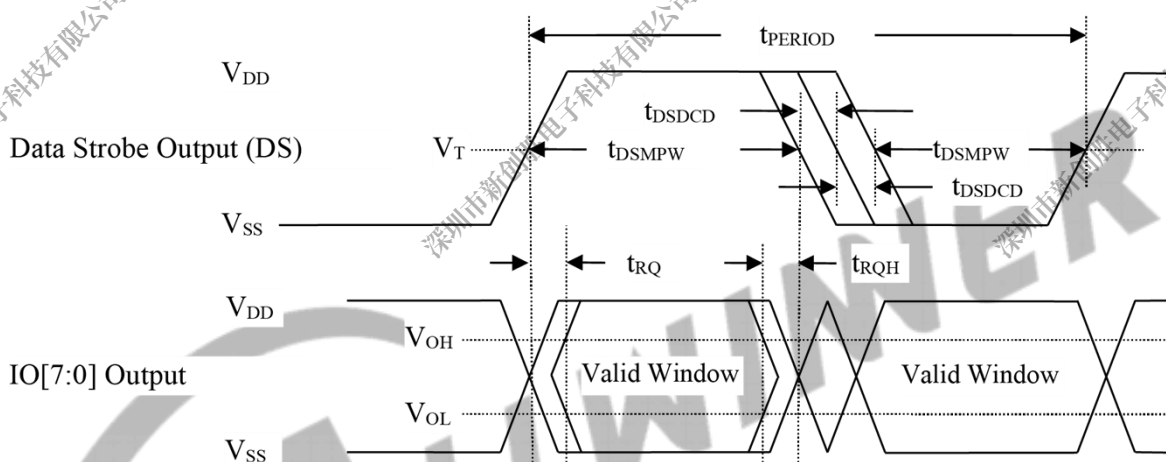
Figure 4-34 xSPI Target Data Output Timing
