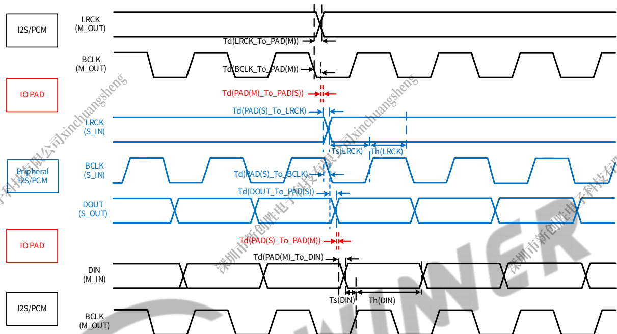
Figure 4-40 Data Input Timing of I2S/PCM in Master Mode
