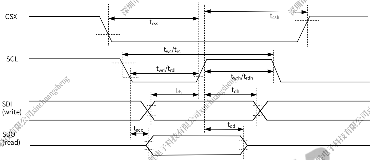
Figure 4-31 DBI 3-line Serial Interface Timing
