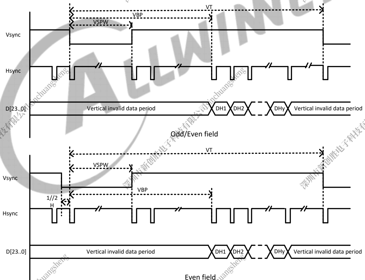
Figure 4-20 HV_IF Vertical Timing
