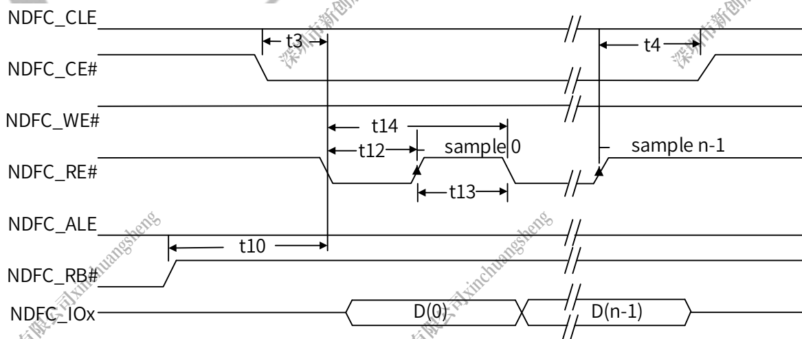
Figure 4-2 Conventional Serial Access Cycle Timing (SAM0)
