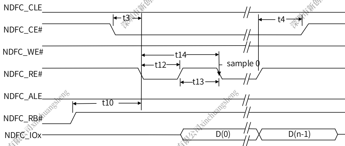
Figure 4-4 Extending EDO Type Serial Access Mode Timing (SAM2)
