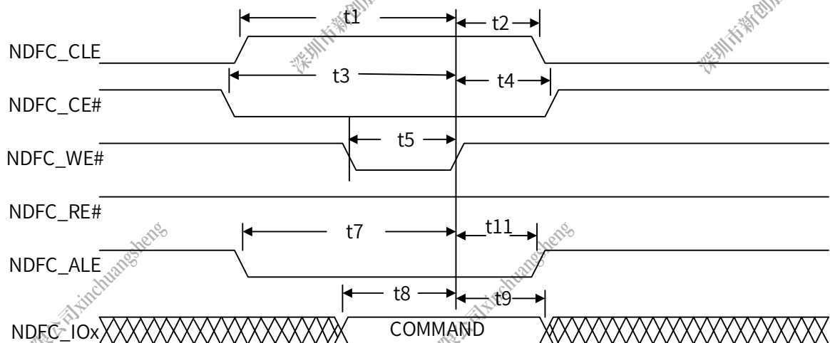
Figure 4-5 Command Latch Cycle Timing
