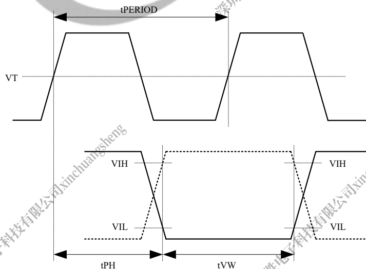
Figure 4-17 SMHC HS200/SDR104 Mode Input Timing Diagram
