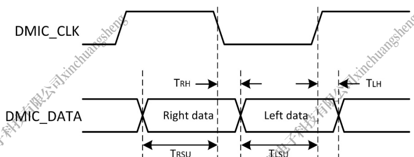
Figure 4-41 DMIC Timing
