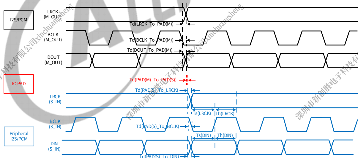
Figure 4-39 Data Output Timing of I2S/PCM in Master Mode
