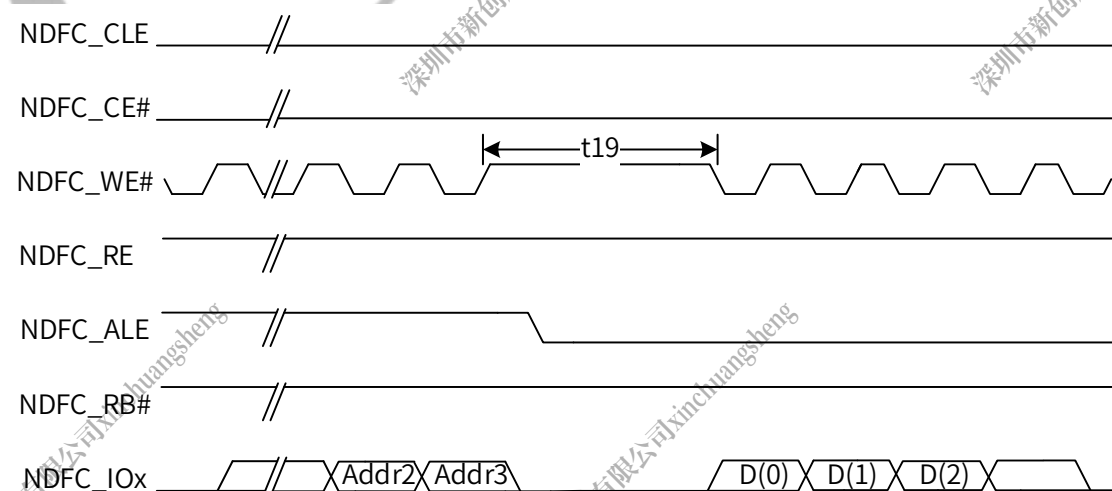
Figure 4-11 Address to Data Loading Timing
