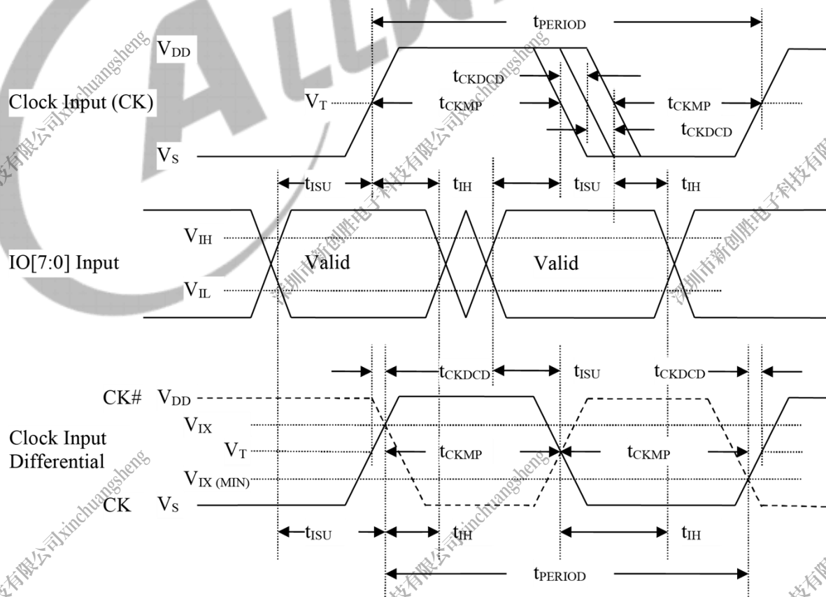
Figure 4-33 xSPI Target Data Input Timing
