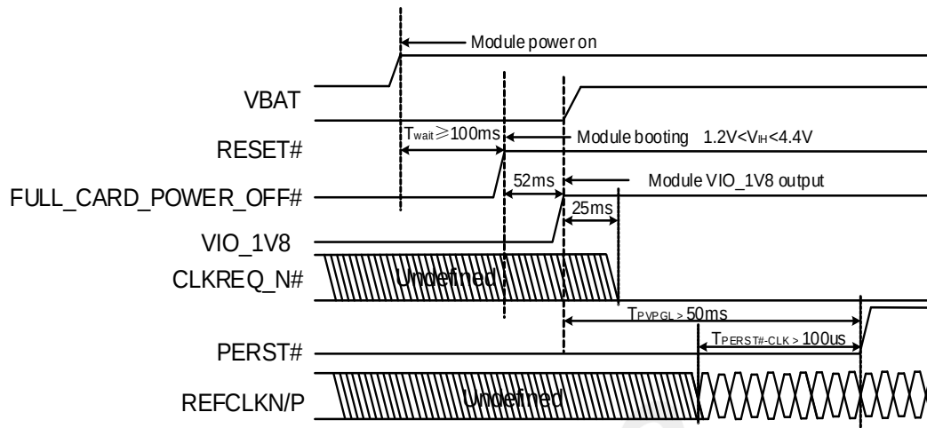
Figure 28: PCIe power-on sequence requirements of module
