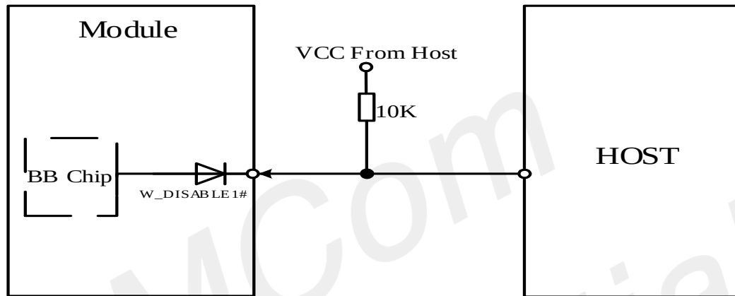
Figure 38: W_DISABLE1# pin reference circuit
