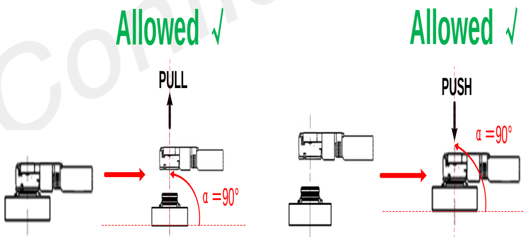
Figure 46: RF cable correct pull and push operation
