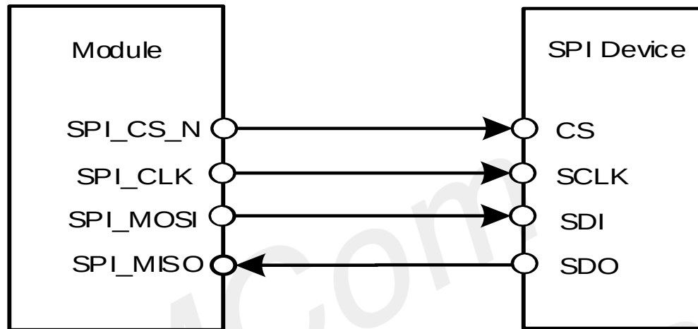
Figure 19: SPI reference circuit
