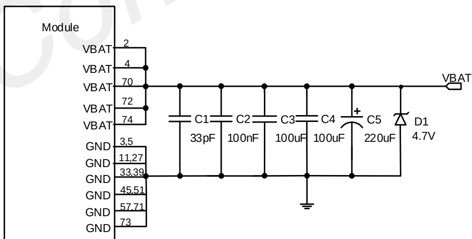
Figure 8: Power supply reference circuit
