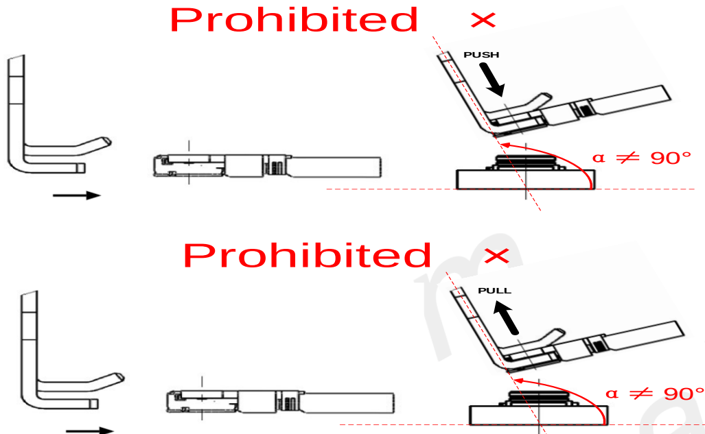
Figure 49: Use RF cable tool error pull and push operation
