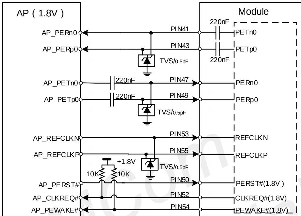
Figure 26: PCIe interface reference circuit (EP Mode, PCIe assistant signal is 1.8V version)
