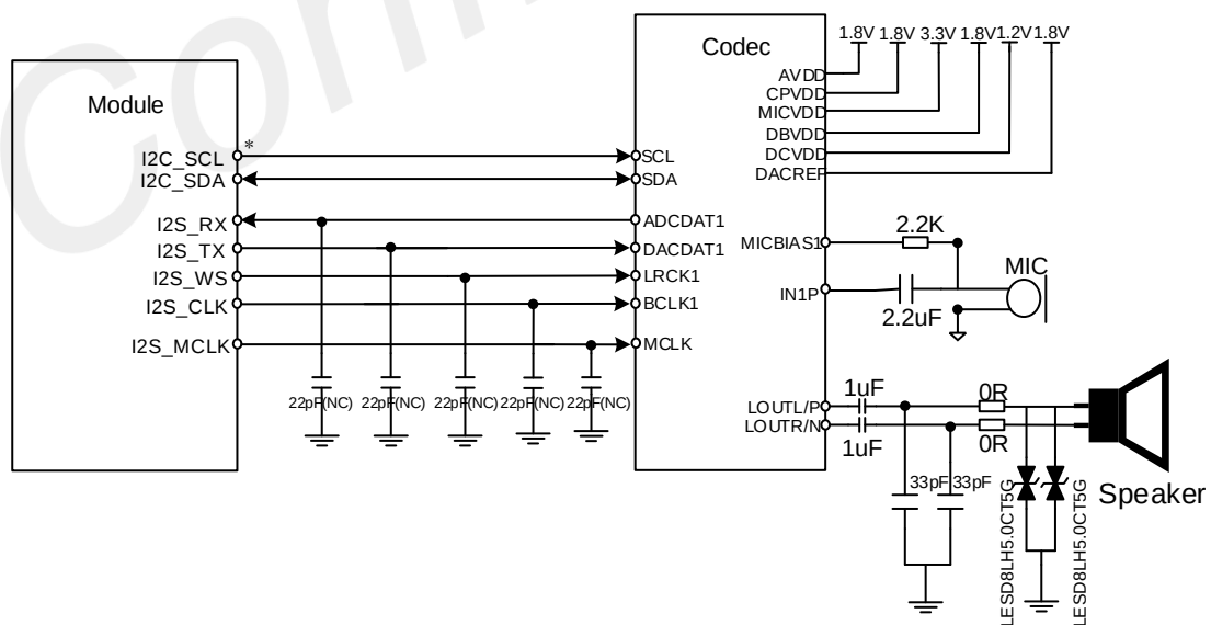
Figure 36: Audio codec diagram circuit
