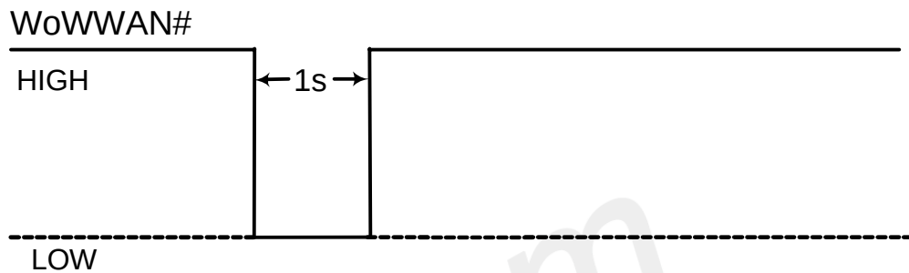
Figure 20: WoWWAN# signal level at SMS and URC report
