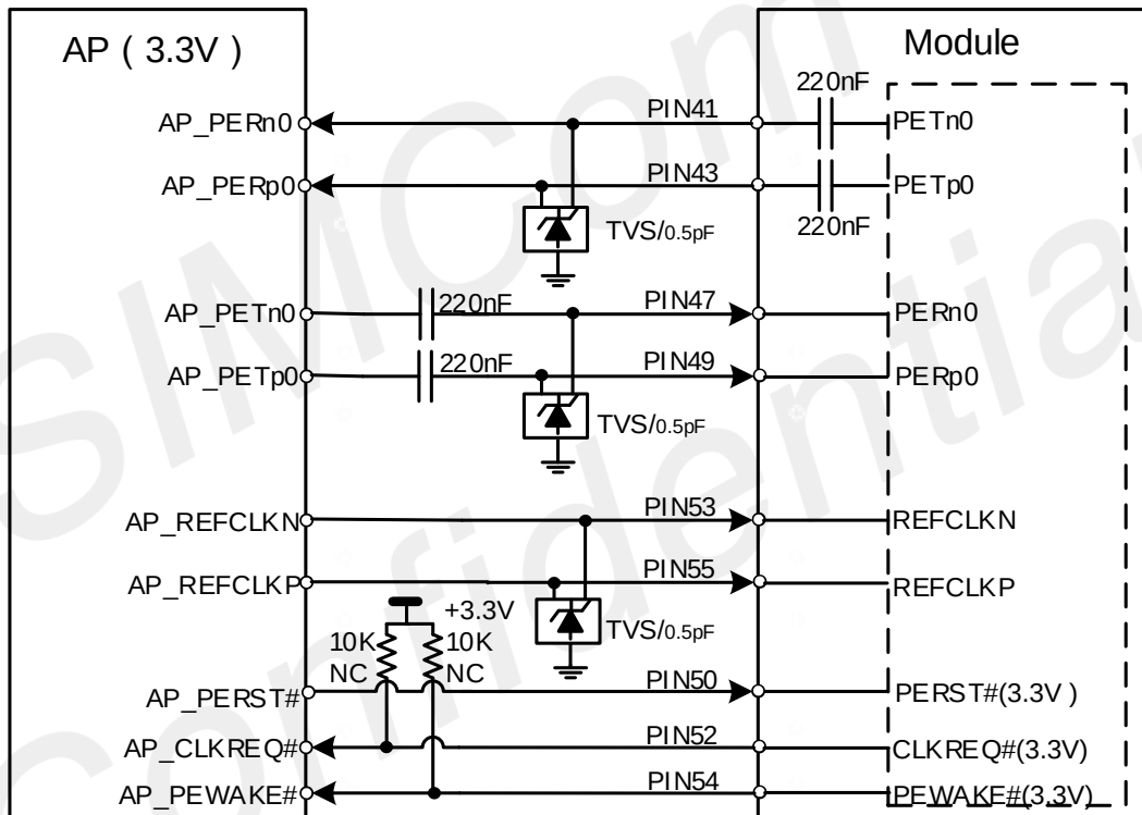
Figure 25: PCIe interface reference circuit (EP Mode, PCIe assistant signal is 3.3V version)
