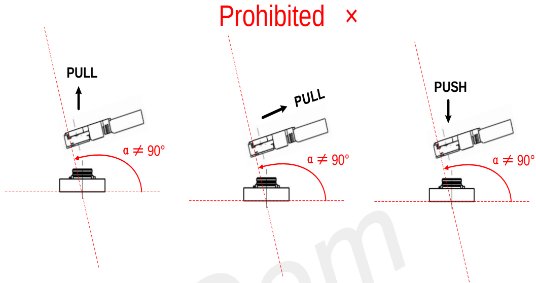
Figure 47: RF cable error pull and push operation
