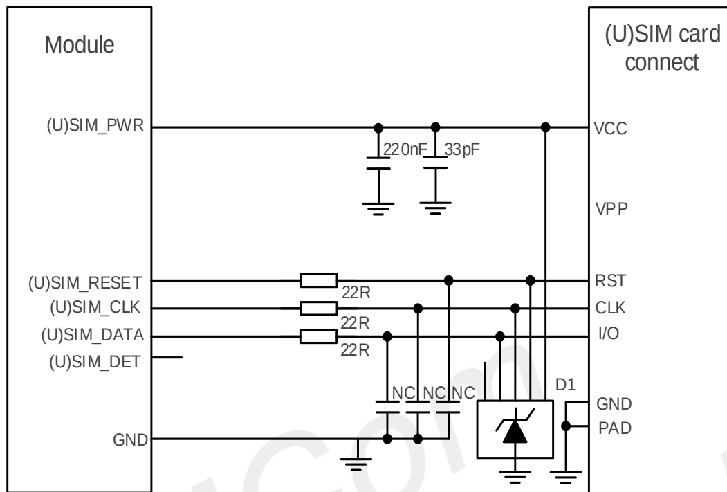
Figure 34: Without CD pin (U)SIM card reference circuit
