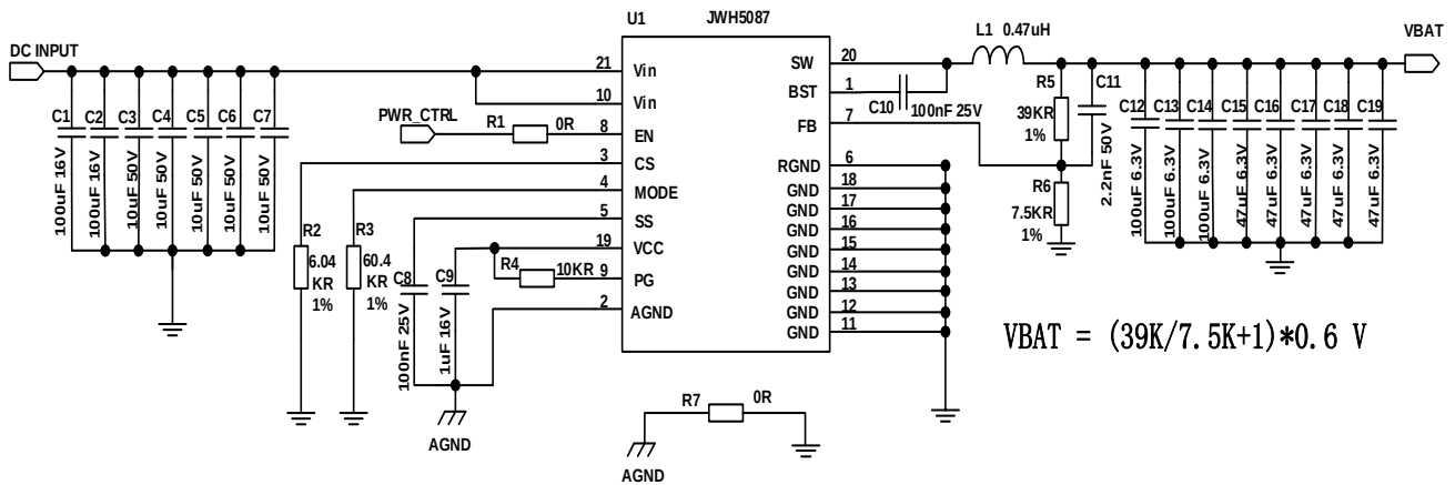
Figure 12: Switching mode power supply reference circuit for mmW module (SIM8380G-M2)
