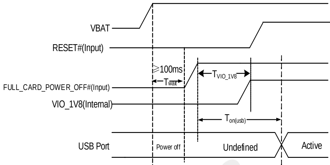
Figure 14: Power on sequence
