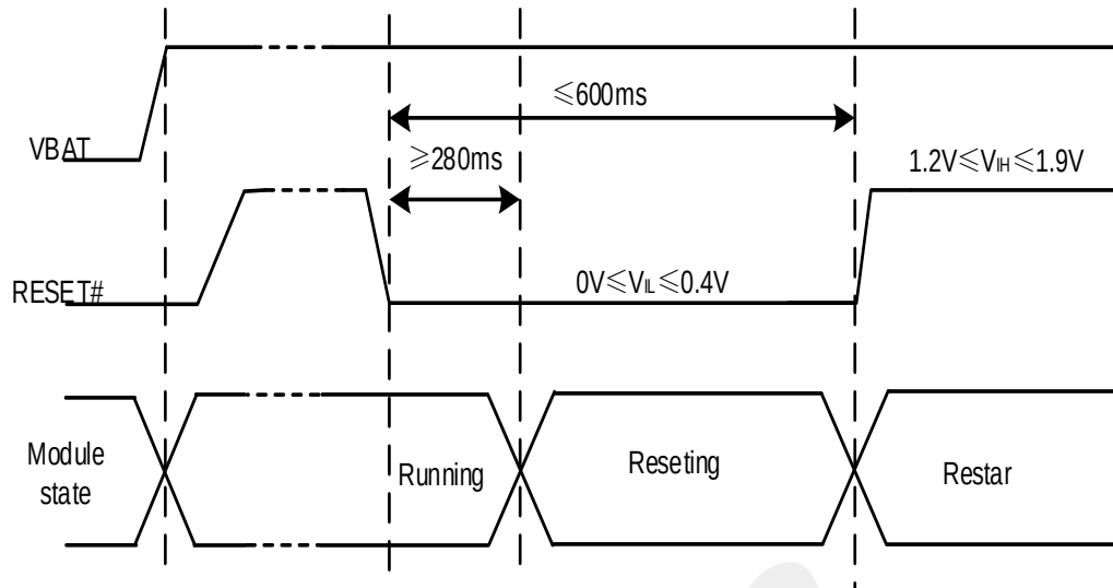
Figure 17: The reset timing sequence of the module
