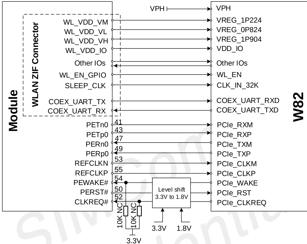
Figure 29: The module connect W82 reference circuit (PCIe assistant signal is 3.3V version)
