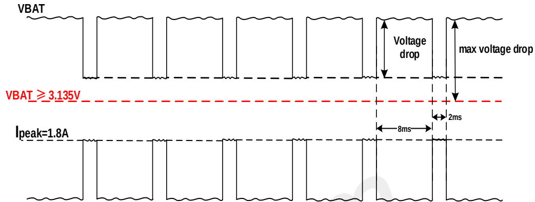
Figure 7: Voltage drop and maximum current consumption
