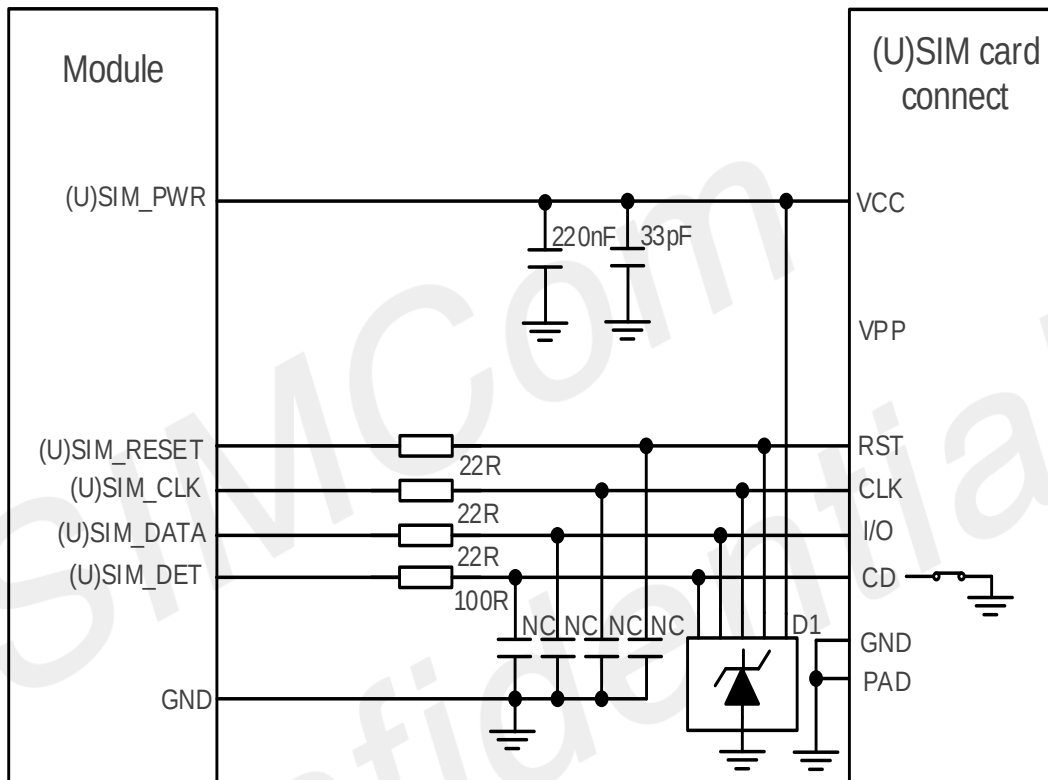
Figure 32: Always close (U)SIM card reference circuit
