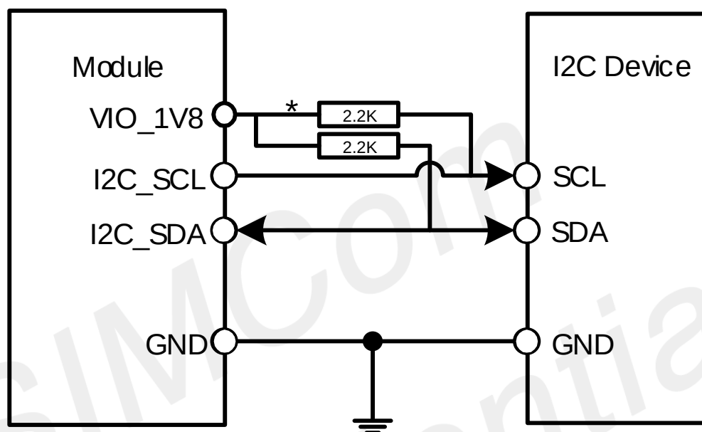
Figure 18: I2C reference circuit
