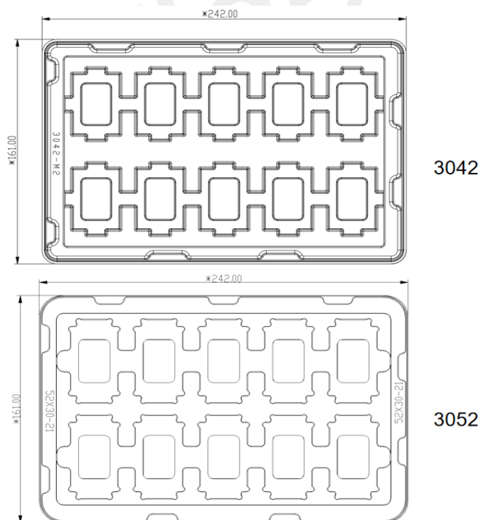
Figure 55: Tray view of the module
