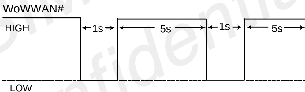
Figure 21: WoWWAN# signal level at received voice call but not be answered
