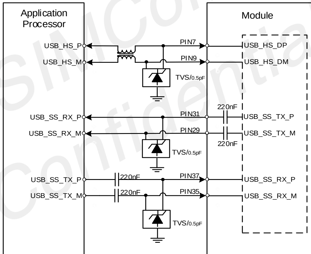
Figure 23: USB reference circuit
