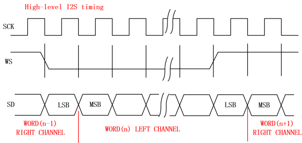
Figure 35: I2S timing
