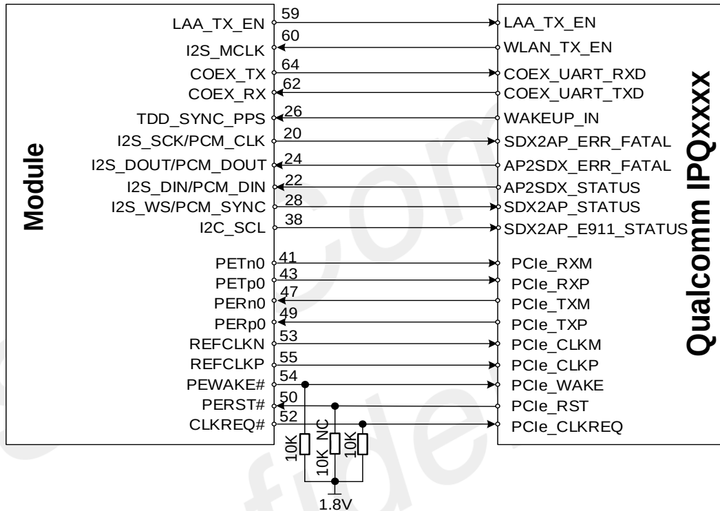
Figure 31: The module connect IPQxxxx reference circuit (1.8V PCIe assistant signal version)
