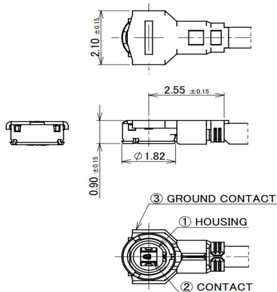
Figure 45: Mechanical information of RF plug
