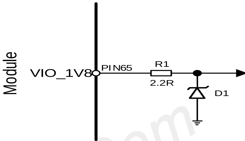
Figure 9: Power supply reference circuit
