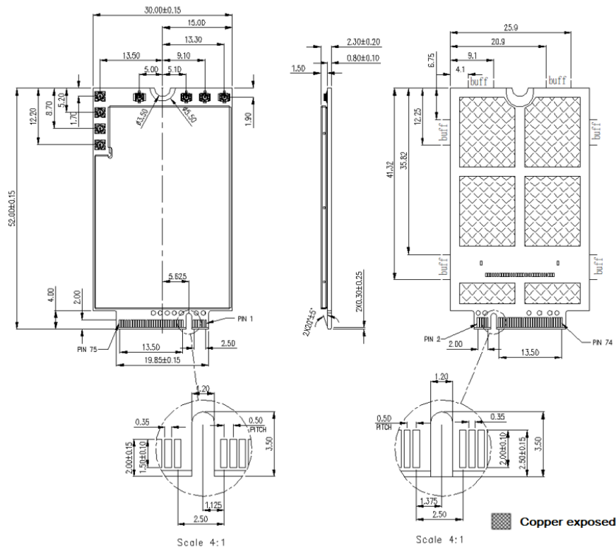
Figure 6: Dimensions of the module (unit: mm)
