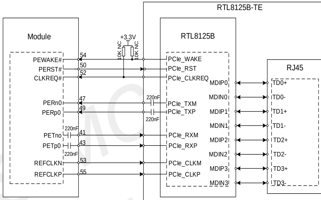
Figure 30: The module connect RTL8125B-TE reference circuit (3.3V PCIe assistant signal version)
