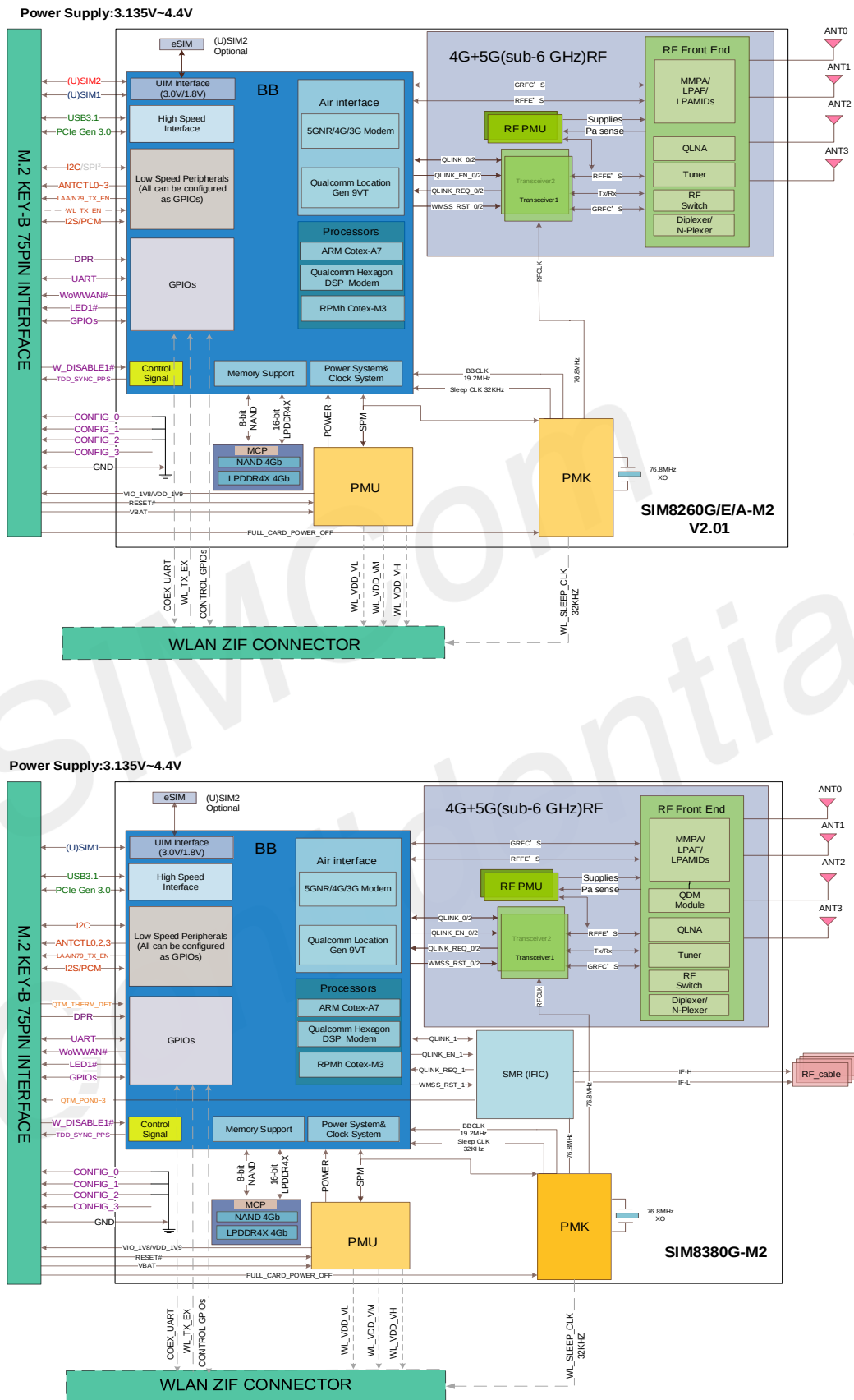
Figure 2: Block diagram
