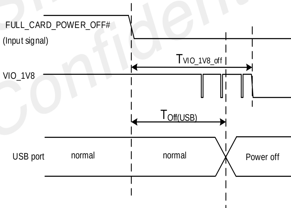
Figure 15: Power off sequence
