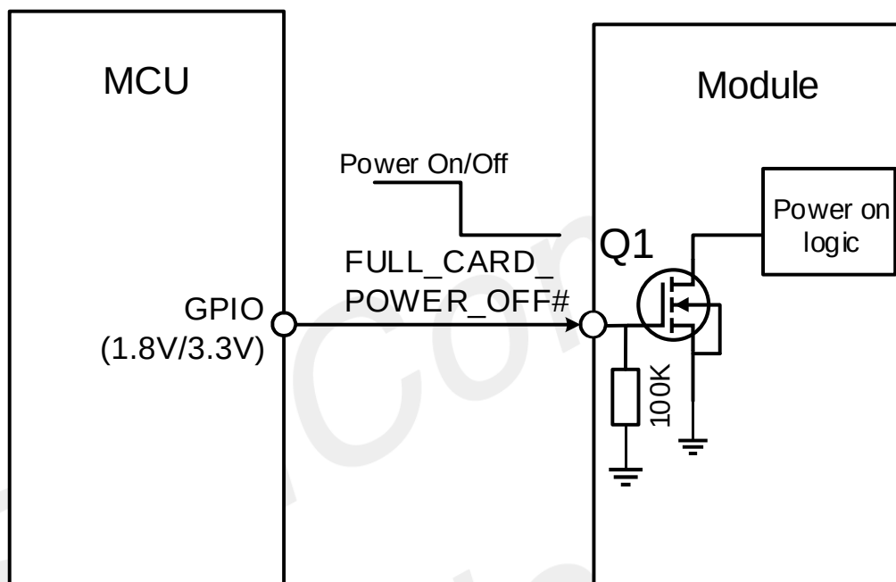
Figure 13: Reference power on/off circuit
