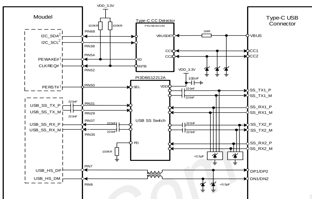
Figure 24: Type-C USB reference circuit with CC detector
