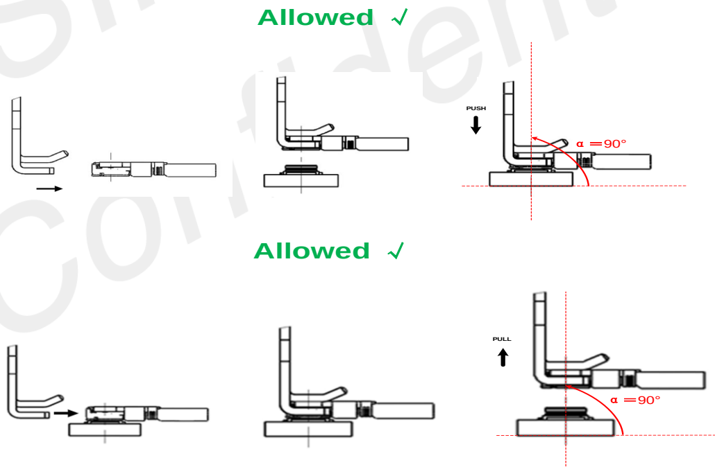
Figure 48: Use RF cable tool correct pull and push operation
