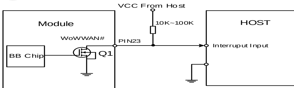
Figure 22: WoWWAN# reference circuit
