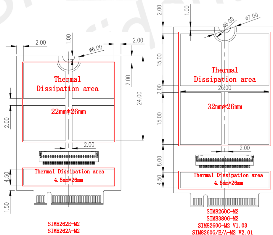
Figure 50: Thermal design diagram
