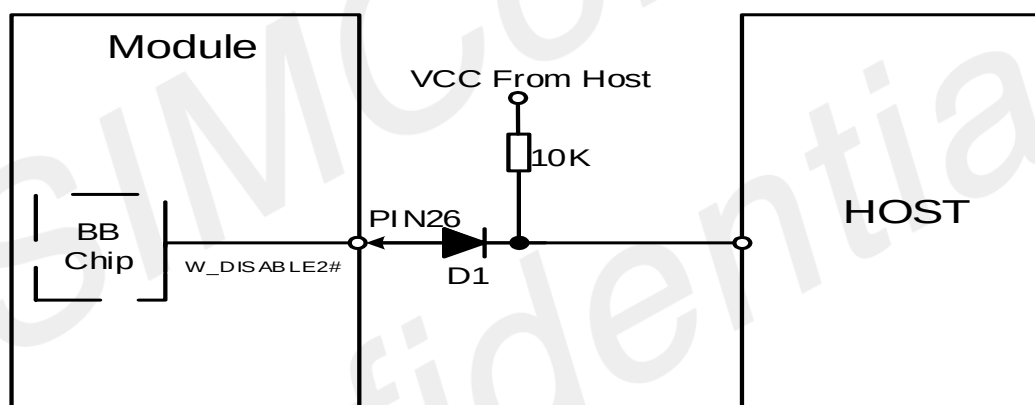
Figure 40: W_DISABLE2# pin reference circuit
