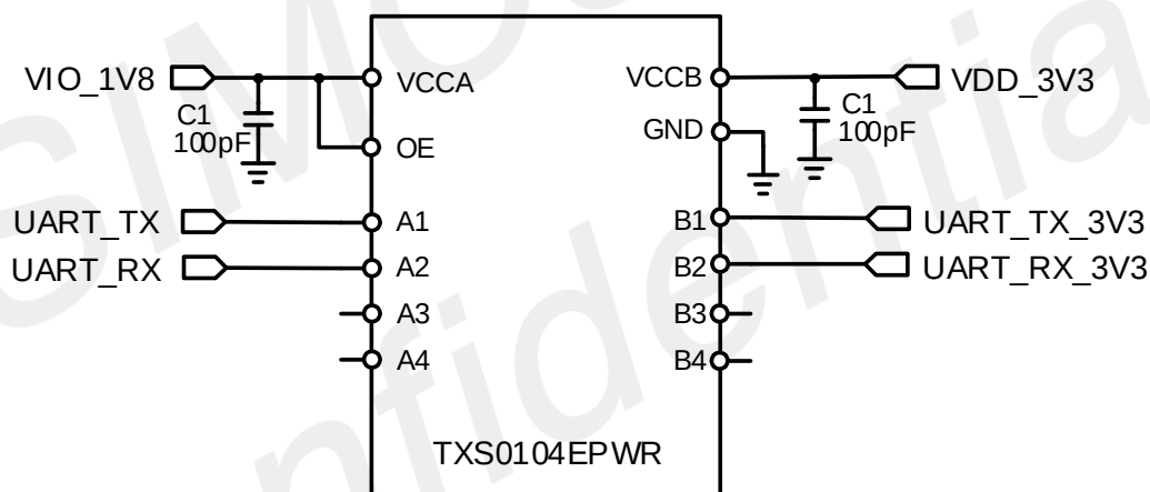
Figure 41: UART level conversion circuit
