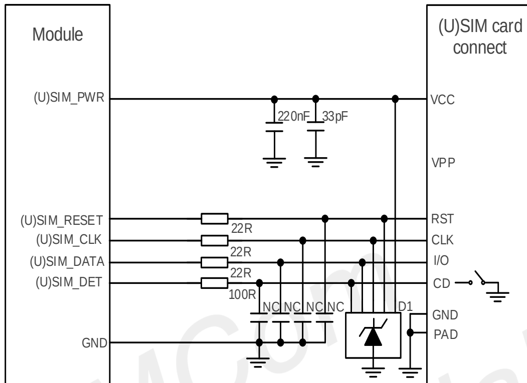
Figure 33: Always open (U)SIM card reference circuit
