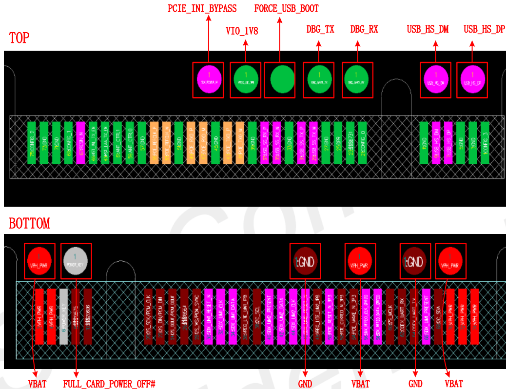
Figure 5: Test point of SIM826XX/SIM8X80-M2 series module
