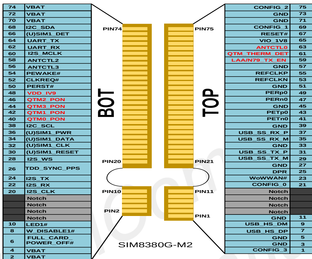
Figure 3: Pin assignment
