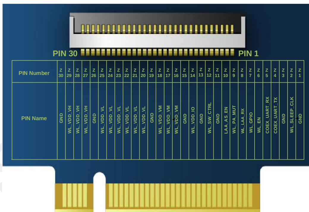
Figure 4: Pin map of WLAN ZIF connector interface
