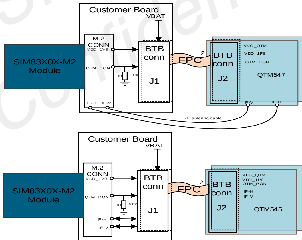
Figure 42: The connection diagram of module and mmW module
