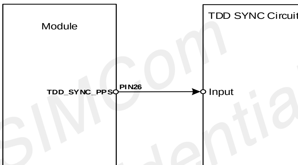
Figure 39: TDD_SYNC_PPS pin reference circuit
