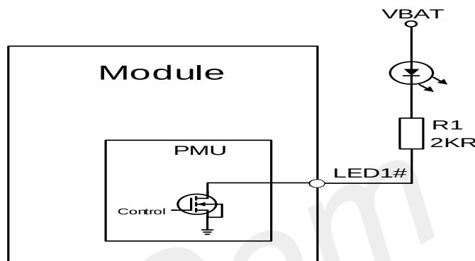
Figure 37: LED1# reference circuit
