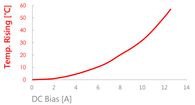
VEFL2C0630-2R2MPA
