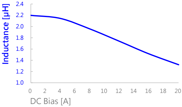
VEFL2C0630-2R2MPA
