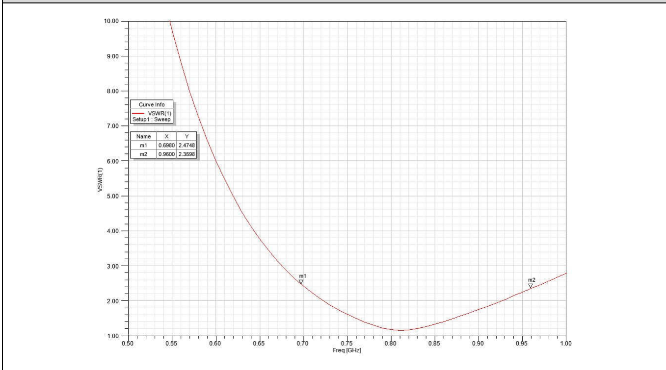
Antenna VSWR on Test Board
