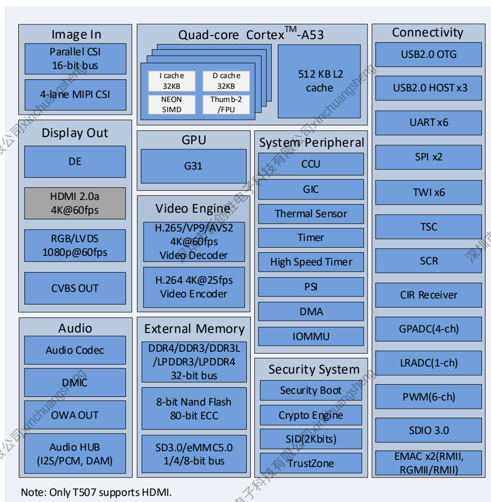
Figure 3-1. T5 Series System Block Diagram
