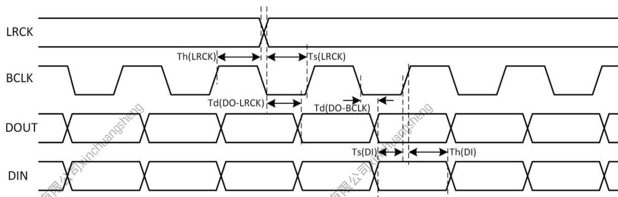
Figure 5-57. I2S/PCM Timing in Slave Mode
