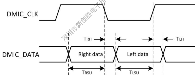
Figure 5-58. DMIC Timing
