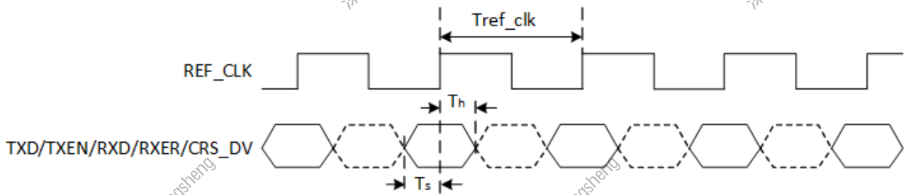
Figure 5-41. RMII Interface Timing
