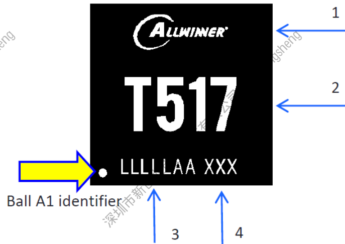
Figure 11-3. T517 Marking
