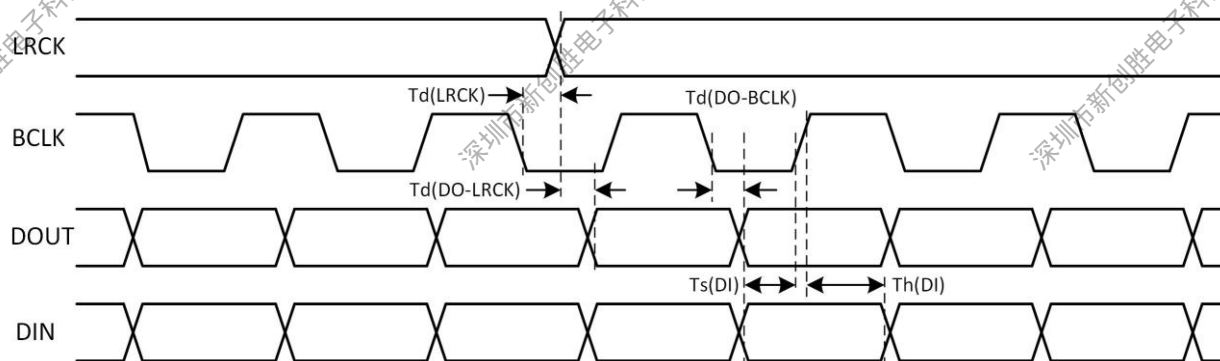
Figure 5-56. I2S/PCM Timing in Master Mode
