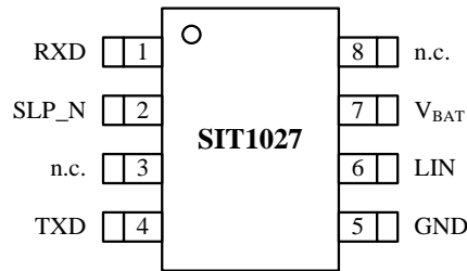
Fig 2. SIT1027 pin configuration diagrams
