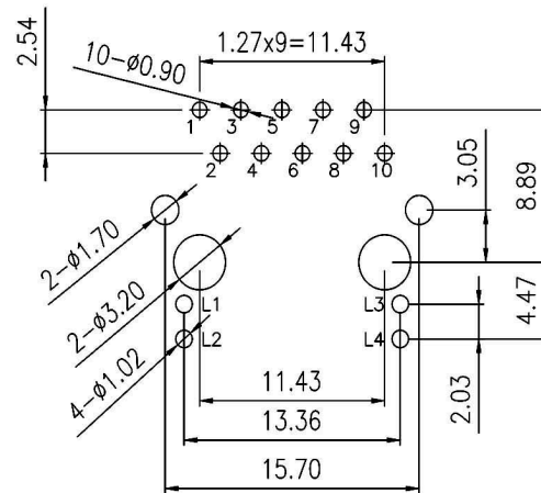
PCB LAYOUT
