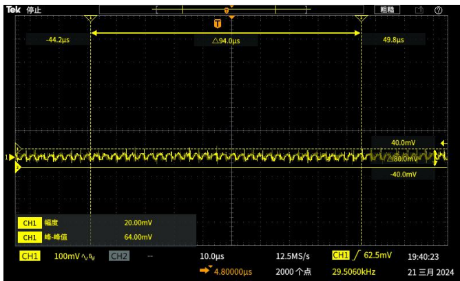
Output ripple (12V /2.5A)
