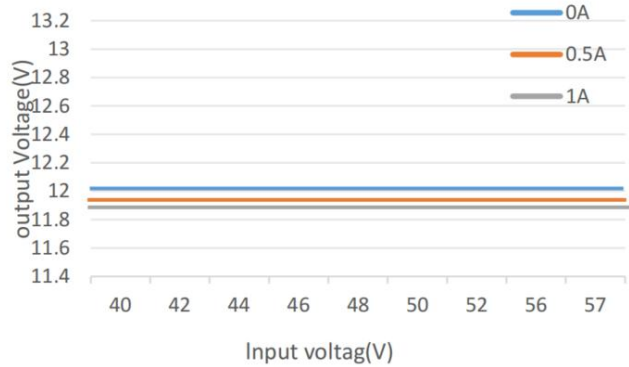
Input voltage & output voltage
