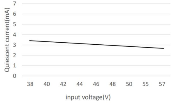
Quiescent current
