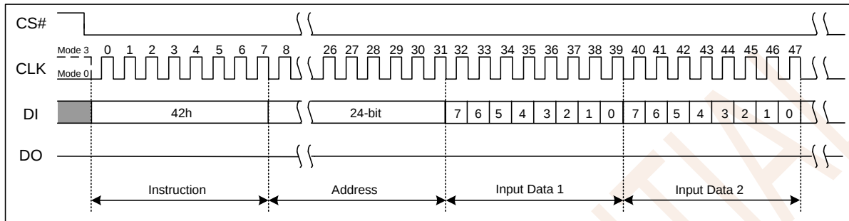
Figure 7.33 Program Security Registers Instruction
