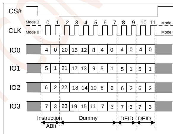
Figure 7.28b Release Power-down / Device ID(QPI Mode)
