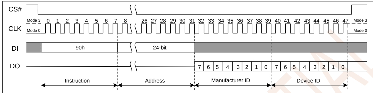
Figure 7.29a Read Manufacturer/Device ID(SPI Mode)
