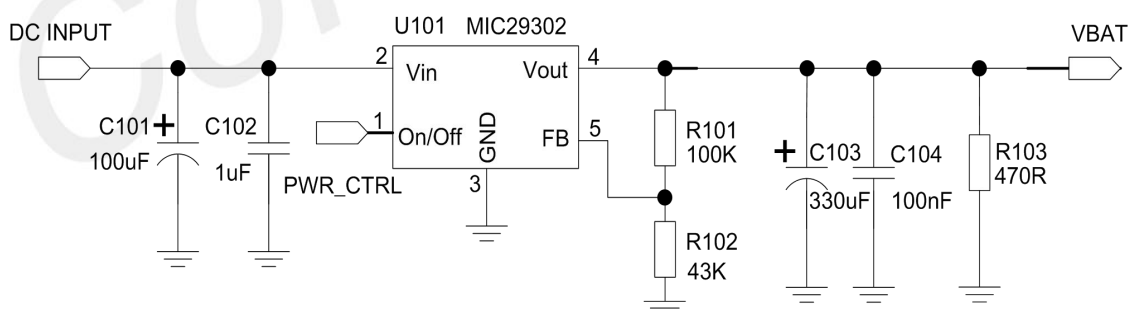
Figure 3: LDO Power Supply Reference Design
