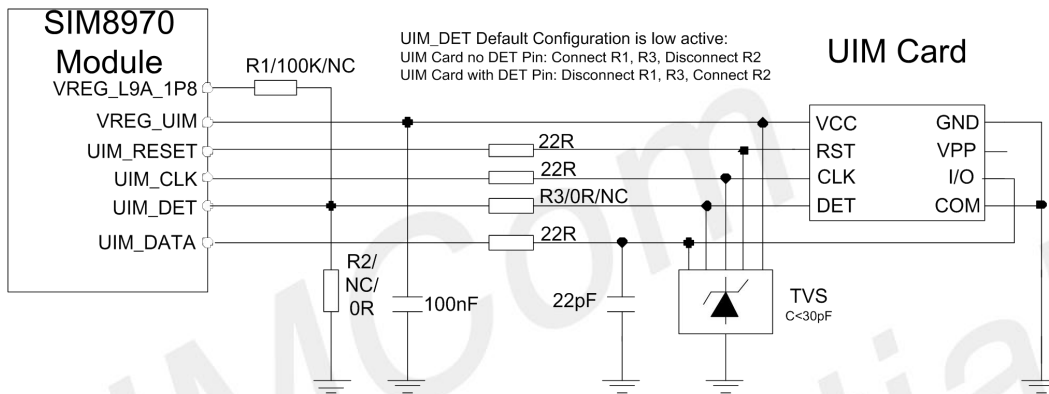
Figure 30: UIM Card Interface Reference Design
