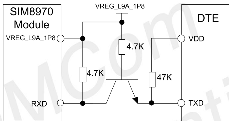
Figure 18: RX Voltage Level Switch Reference Design
