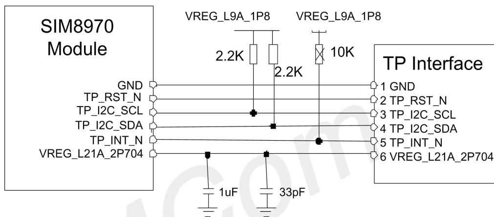
Figure 20: TP Interface Reference Design
