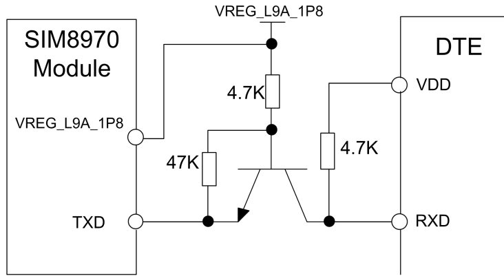
Figure 17: TX Voltage Level Switch Reference Design
