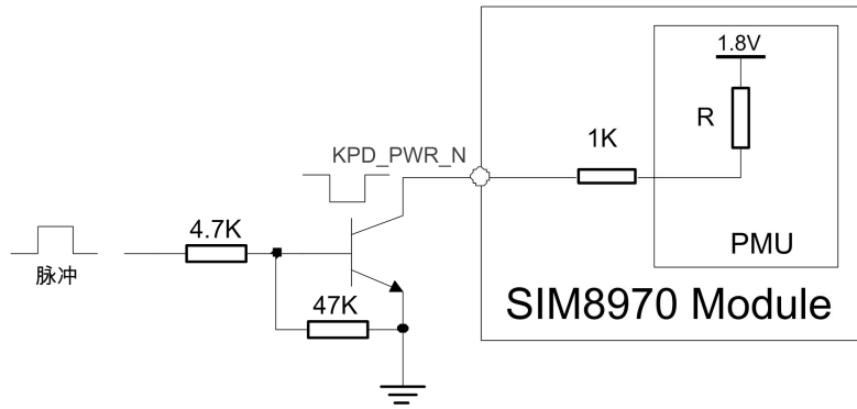
Figure 7: Power On/Off Design with an OC Gate
