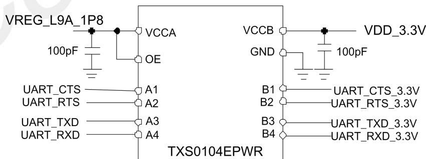
Figure 16: UART Voltage Level Switch Reference Design
