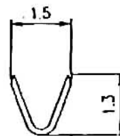
B-B SECTION
