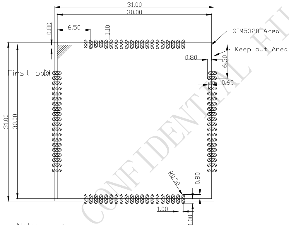
Figure 2: SIM5320 footprint recommendation (Unit: mm)
