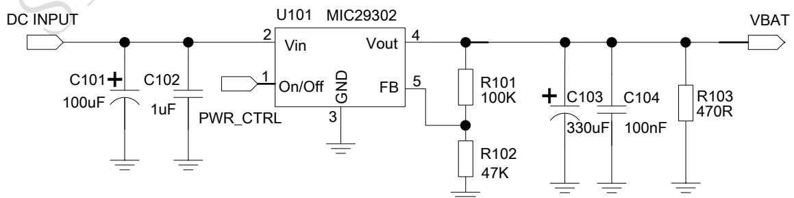
Figure 5: Reference circuit of the LDO power supply
