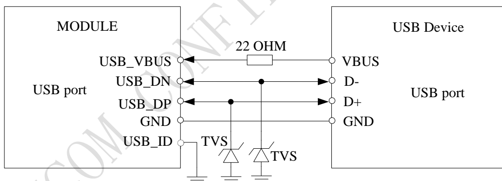
Figure 7: USB interface
