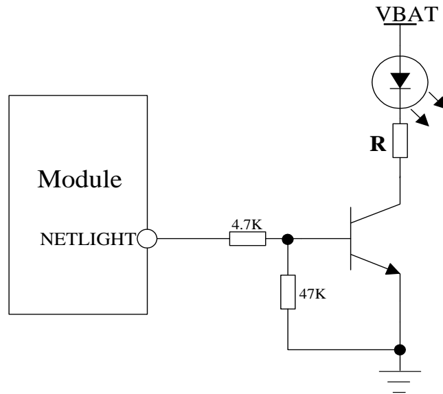
Figure 8: Application circuit
