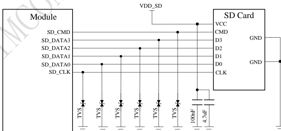
Figure 15: SIM7600 SDC interface for SD card
