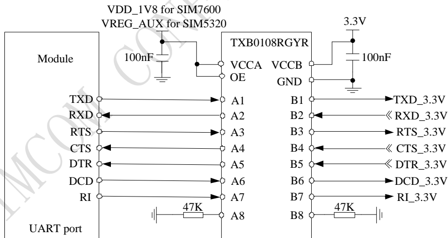
Figure 11: Reference circuit of level shift
