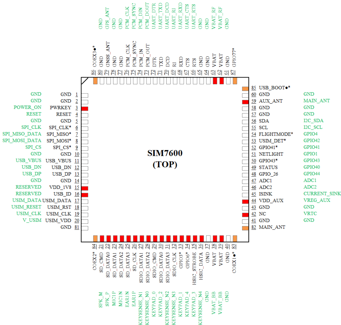
Figure 1: SIM7600 and SIM5320 Pin Assignment
