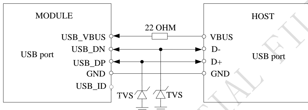
Figure 6: USB interface
