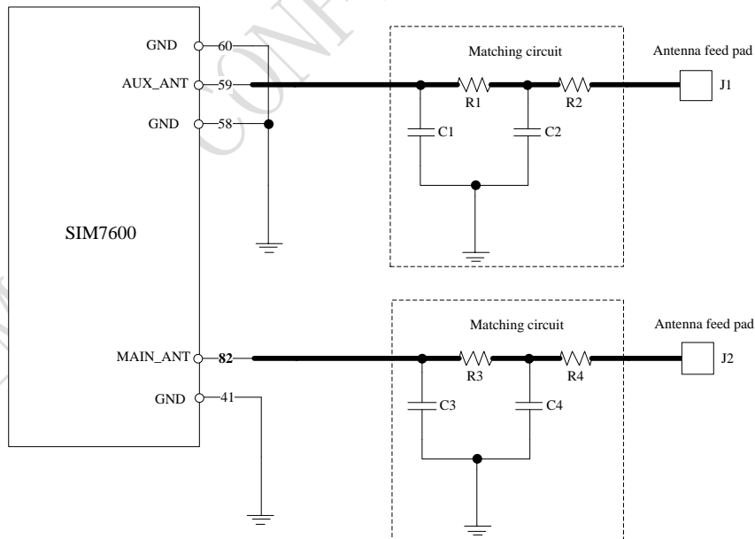
Figure 13: SIM7600 Antenna matching circuit
